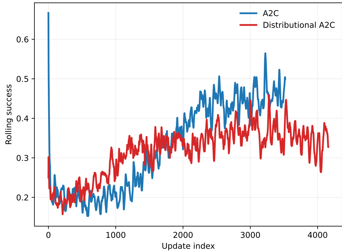
Success Rate
