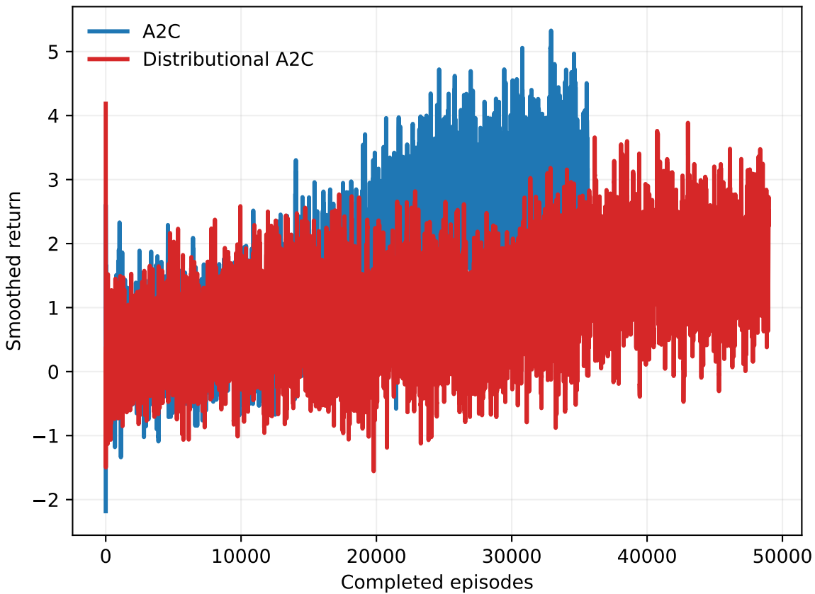
Episode Return
