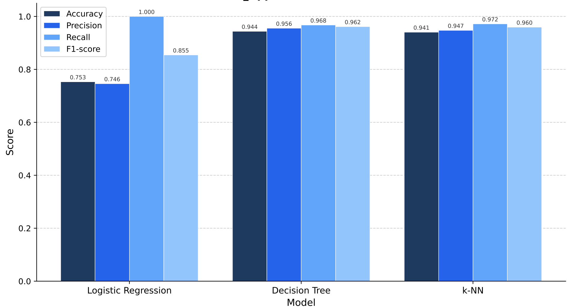
Figure 1: Baseline Model Performance on NYC Yellow Taxi 2025 (is_tipped Classification)
