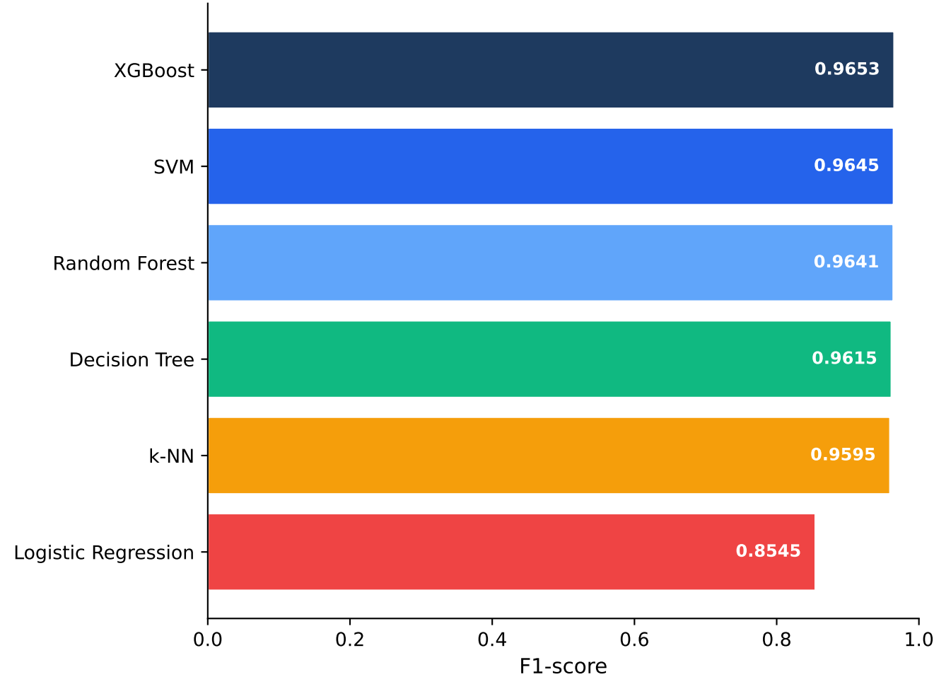
Model Ranking by F1-score
