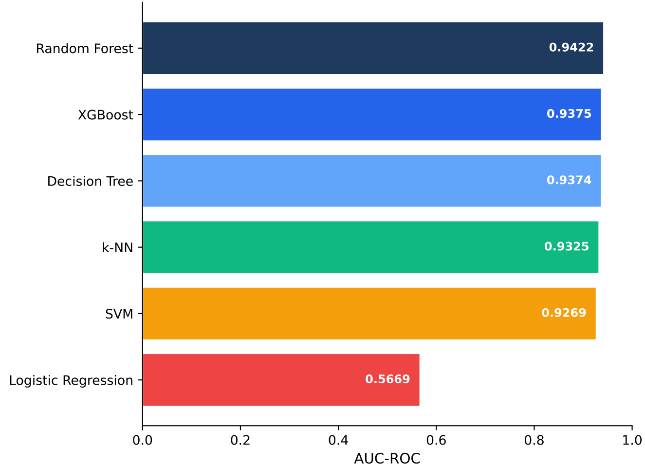
Model Ranking by AUC-ROC
