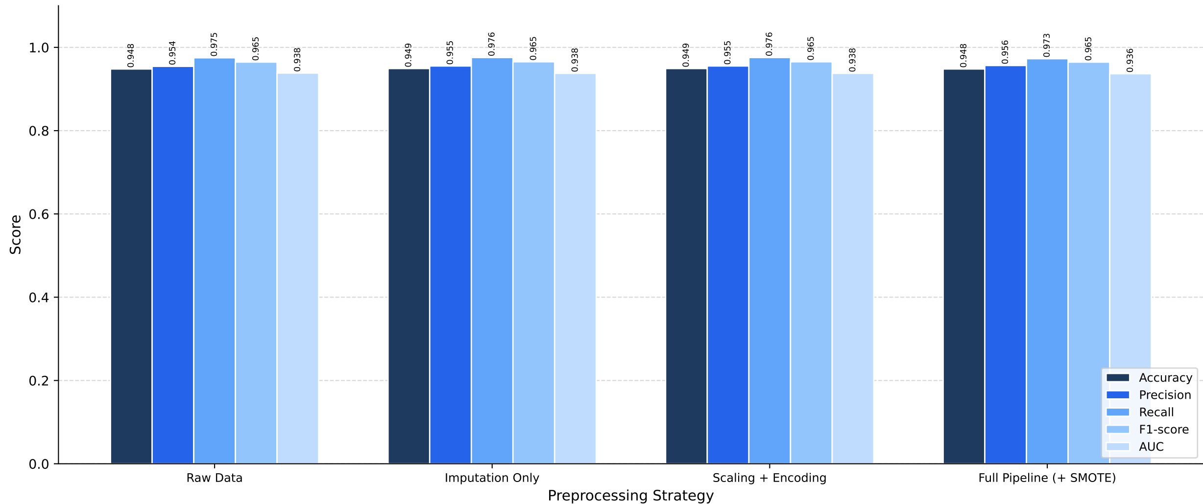
Figure 3: Performance Gains from Different Preprocessing Strategies (XGBoost) NYC Yellow Taxi 2025
