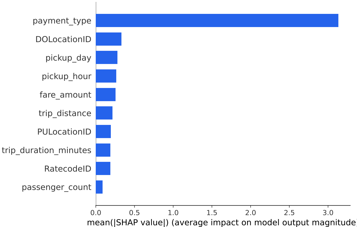
Figure 4b: SHAP Feature Importance — NYC Yellow Taxi 2025
