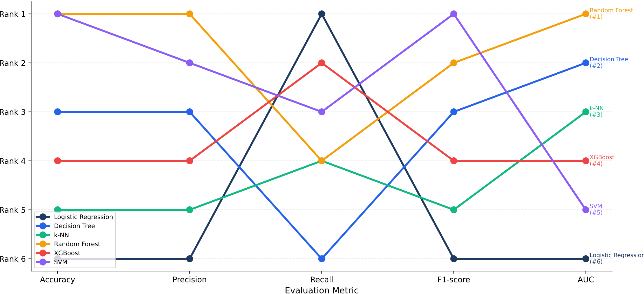
Figure 5: Model Ranking Sensitivity Across Evaluation Metrics NYC Yellow Taxi 2025
