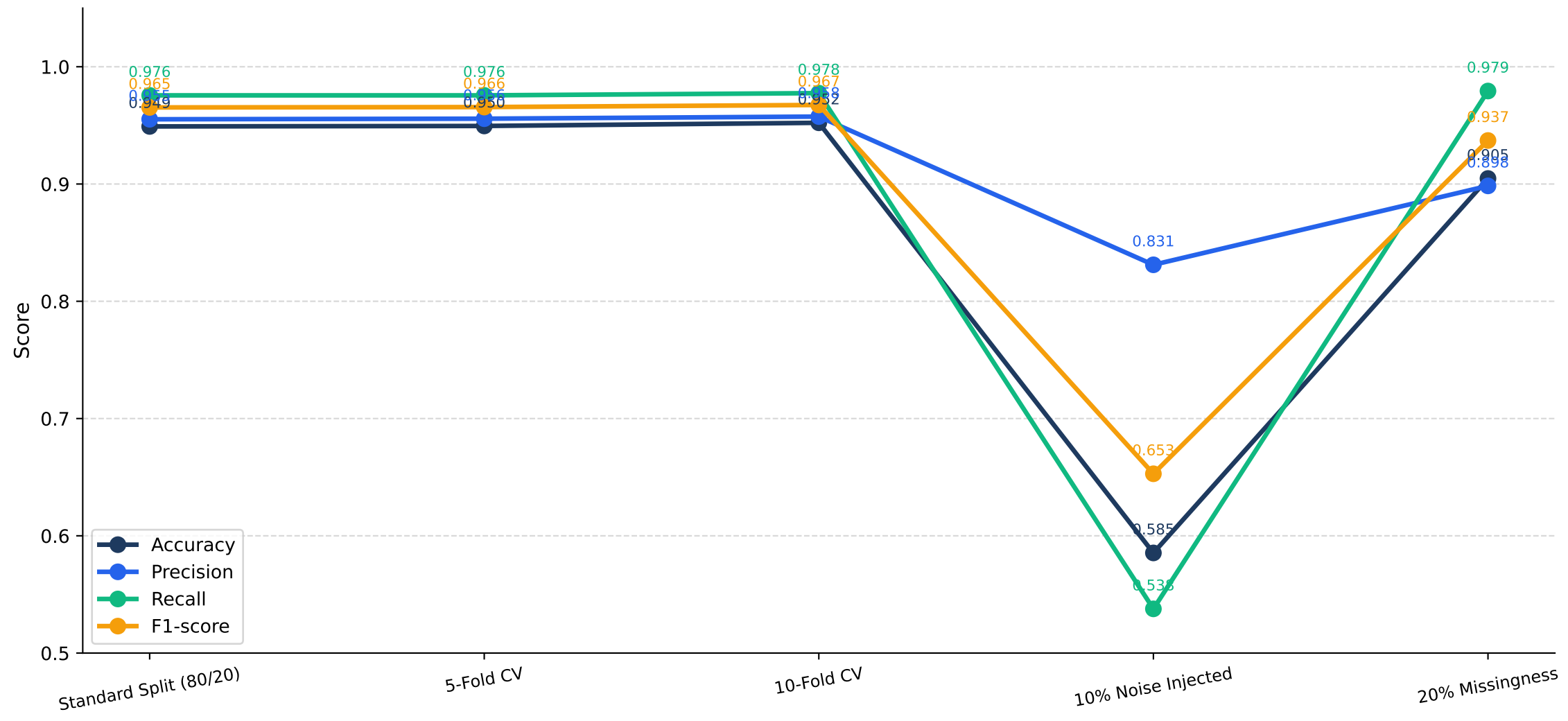
Figure 6: Robustness of XGBoost Under Varying Experimental Conditions NYC Yellow Taxi 2025
