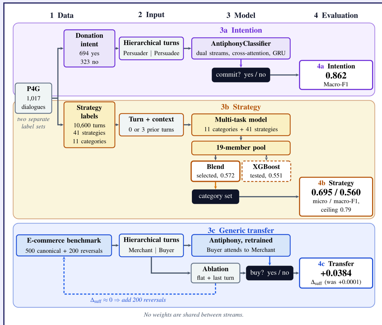
Fig 1 Overall system architecture
