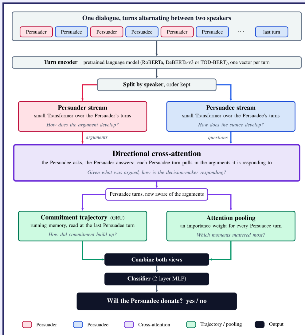
Fig 2 AntiphonyClassifier
