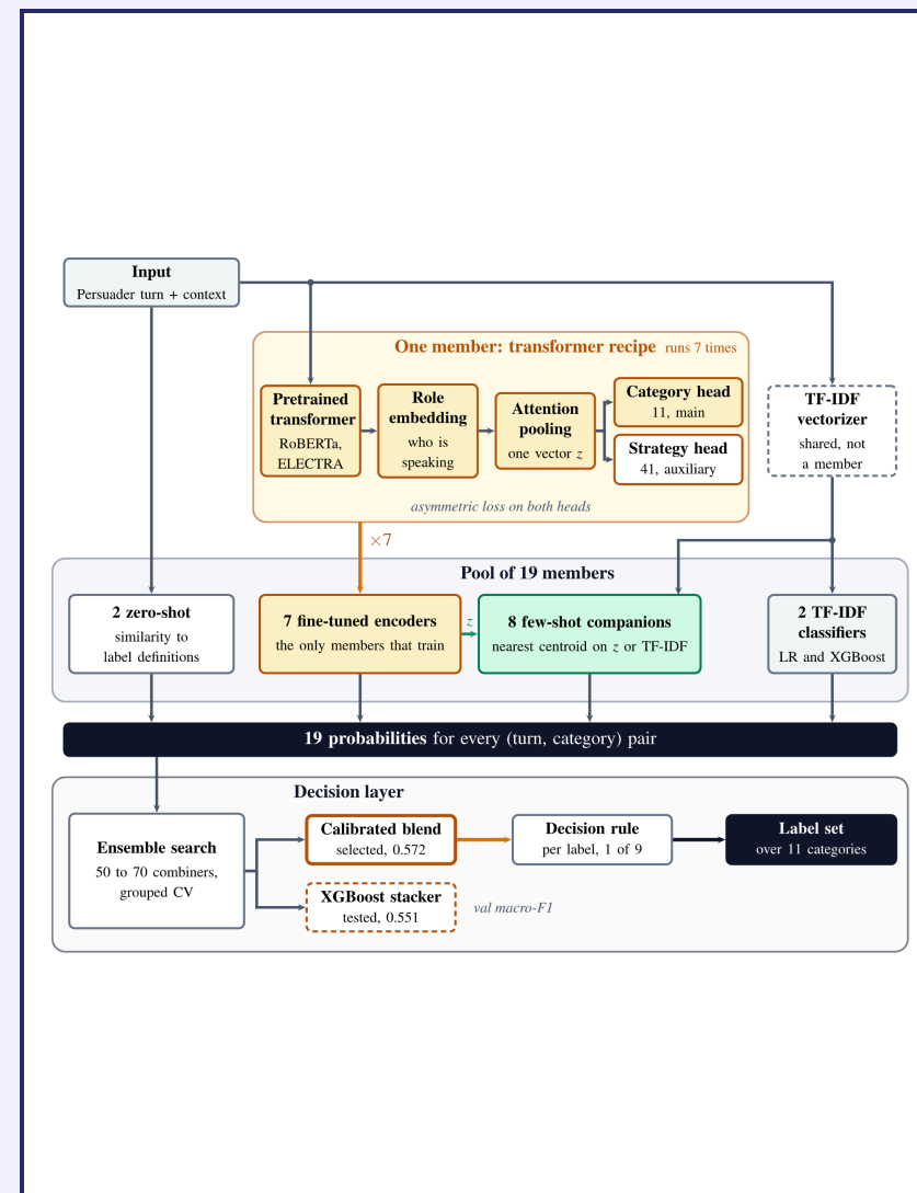
Fig 3 Strategy & category classifier
