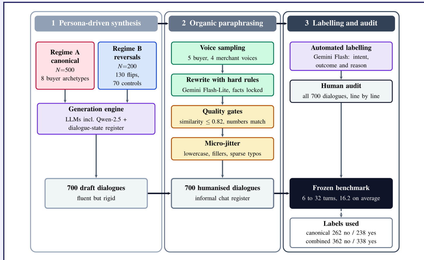
Fig 4 Negotiation benchmark generation
