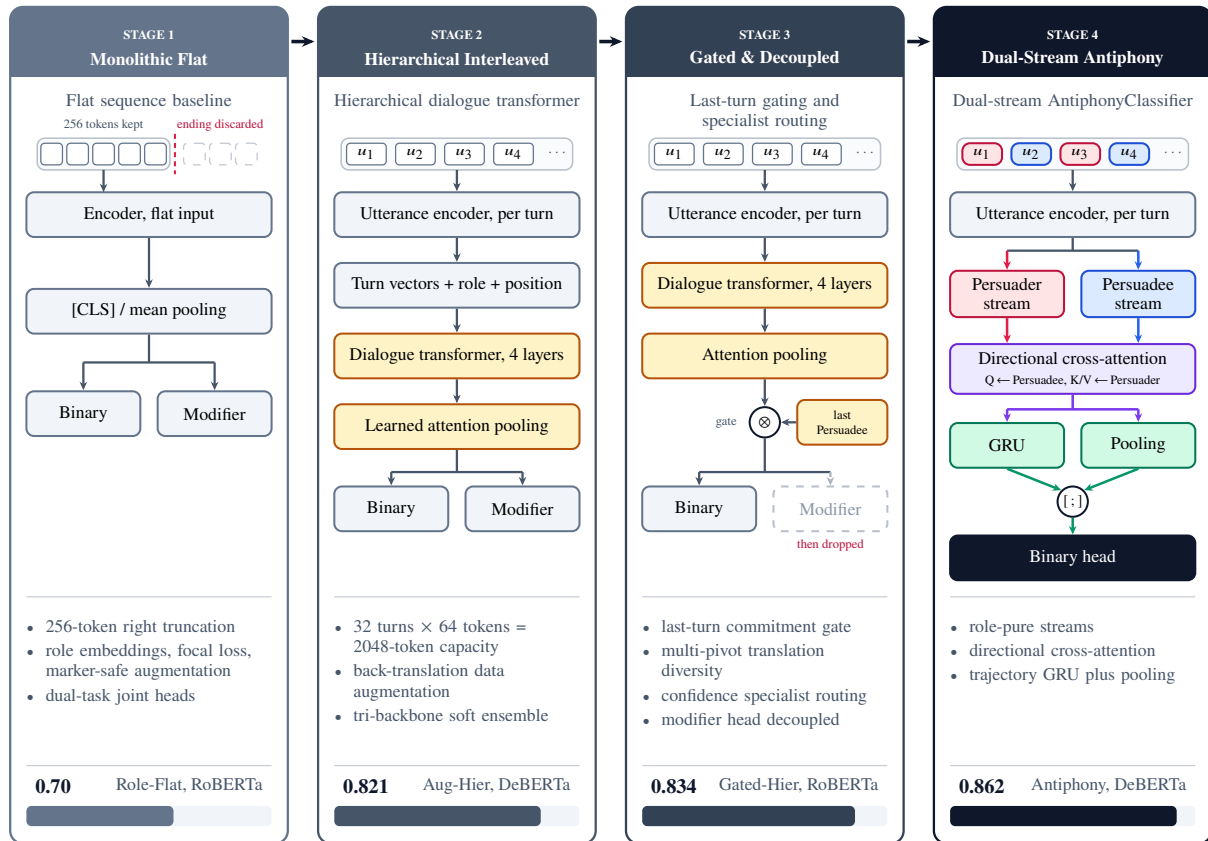
Figure 4.7: Four-stage architectural evolution of intention classification models, depicting key innovations, critical bug diagnoses, and peak test Macro-F1 across stages.
