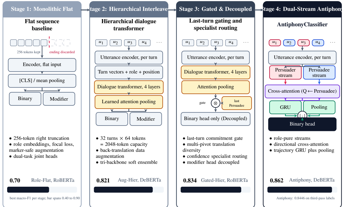
Figure 4.7: Four-stage architectural evolution of intention classification models, depicting key innovations, critical bug diagnoses, and peak test Macro-F1 across stages.
