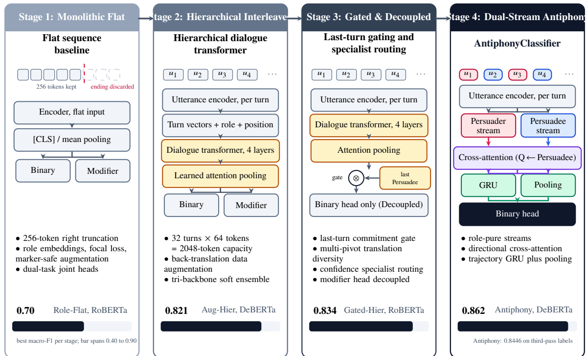
Figure 4.8: Four-stage architectural evolution of intention classification models, depicting key innovations, critical bug diagnoses, and peak test Macro-F1 across stages.
