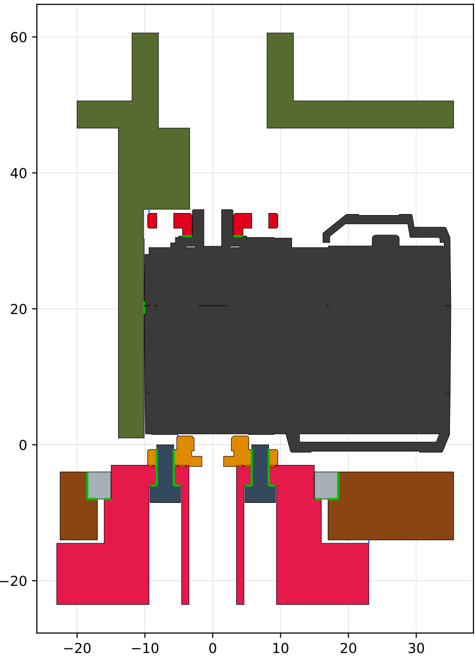
J4 seat, section through the servo axis (servo frame, mm)
