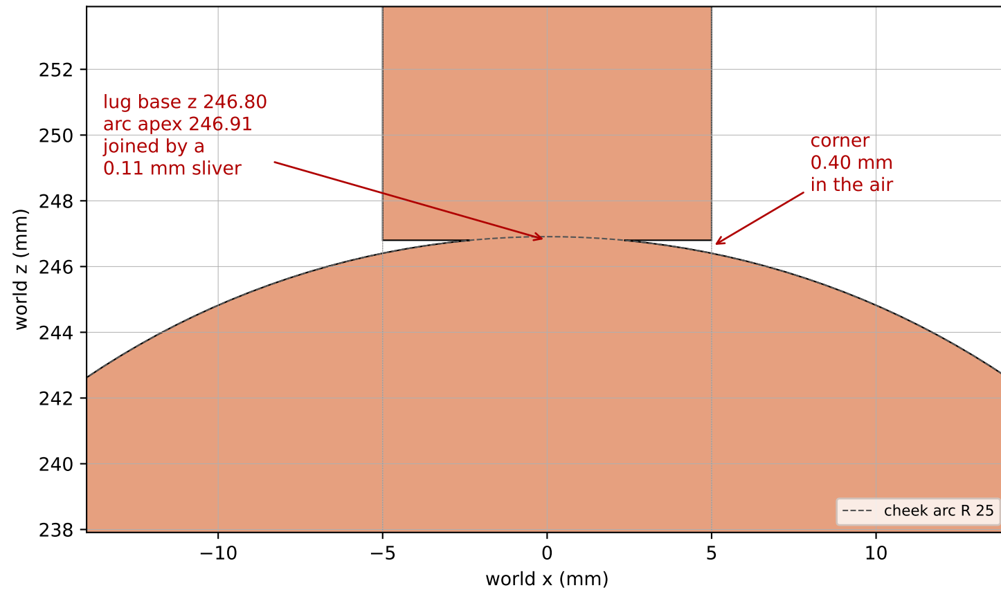
rev I (released) -- +y lug (drive cheek) joint area 35.5 mm2 (lug section 10 x 7.5 = 75 mm2)
