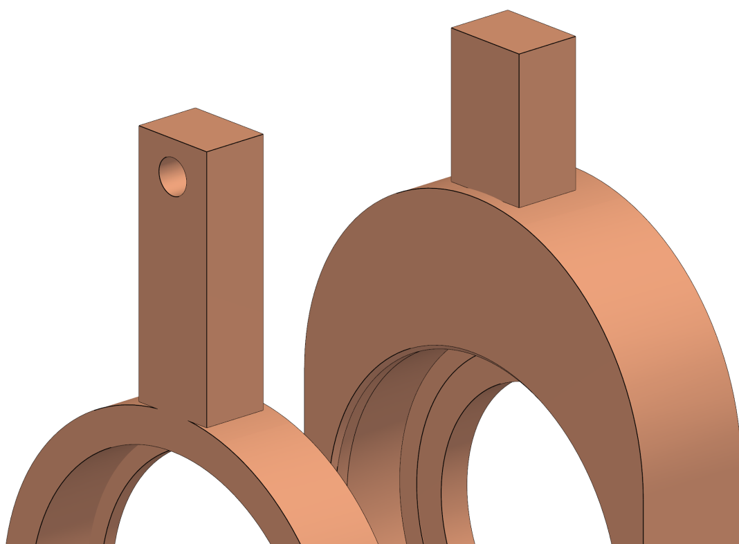
rev I (released) -- both lugs, 3D
