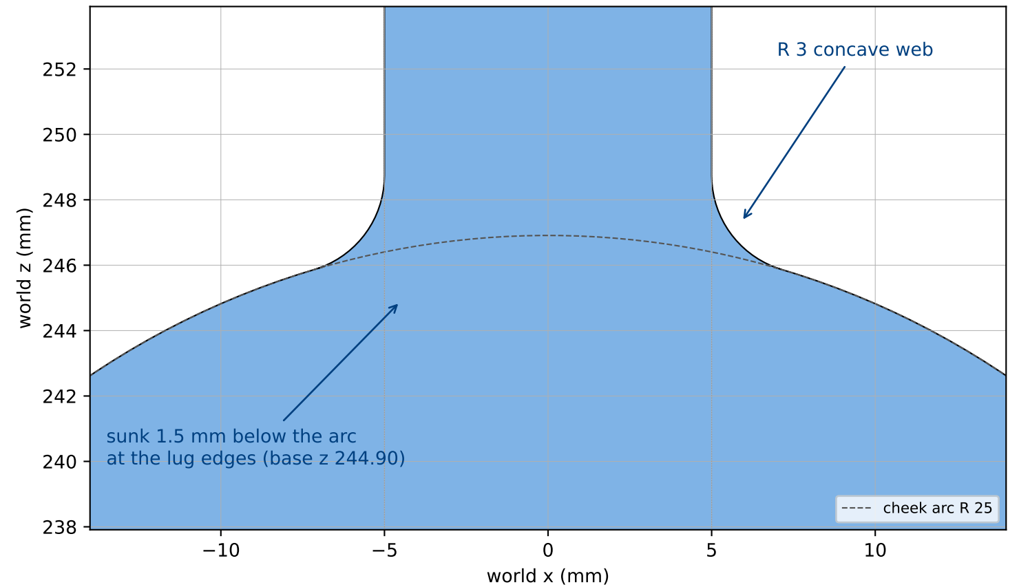
rev I.1 (fixed) -- +y lug (drive cheek) joint area 136.1 mm2 (lug section 10 x 7.5 = 75 mm2)
