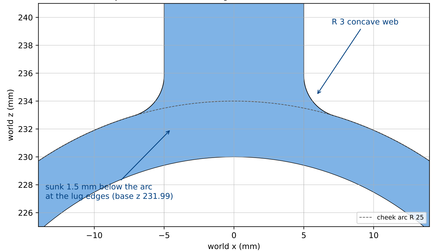
rev I.1 (fixed) -- -y lug (idle cheek) joint area 136.1 mm2 (lug section 10 x 7.5 = 75 mm2)
