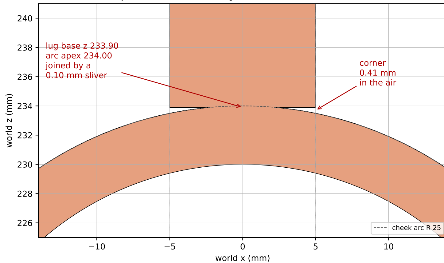
rev I (released) -- -y lug (idle cheek) joint area 33.8 mm2 (lug section 10 x 7.5 = 75 mm2)
