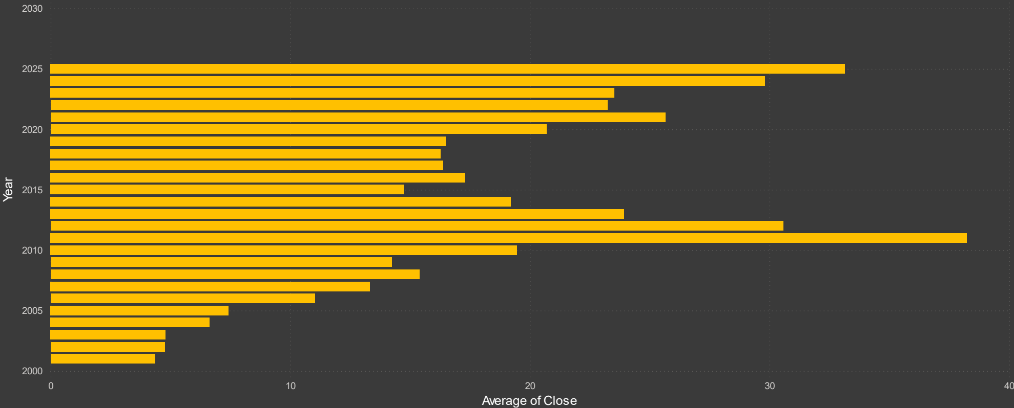
Average of Close by Year
