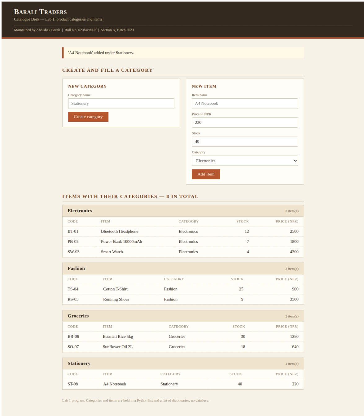
Figure 2: Lab 1 output. 'Stationery' was created and 'A4 Notebook' was added to it, so the catalogue now shows four categories and eight items.
