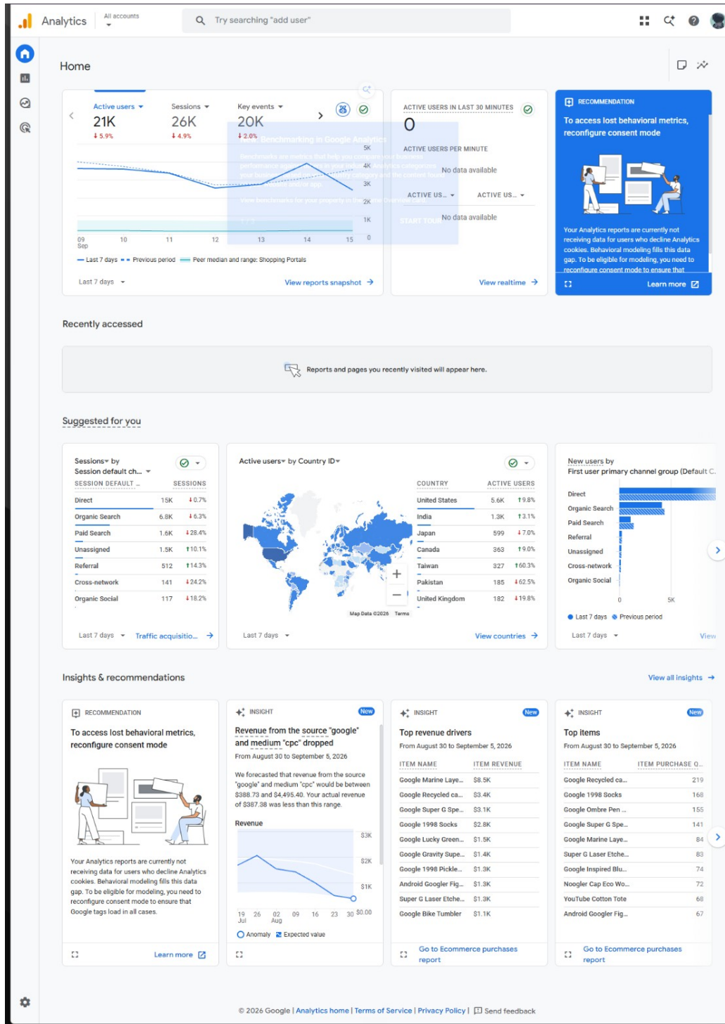
Figure 13: GA4 Home for the Google Merchandise Store demo: about 21K active users, 26K sessions and 20K key events over 7 days, with the live world map.
