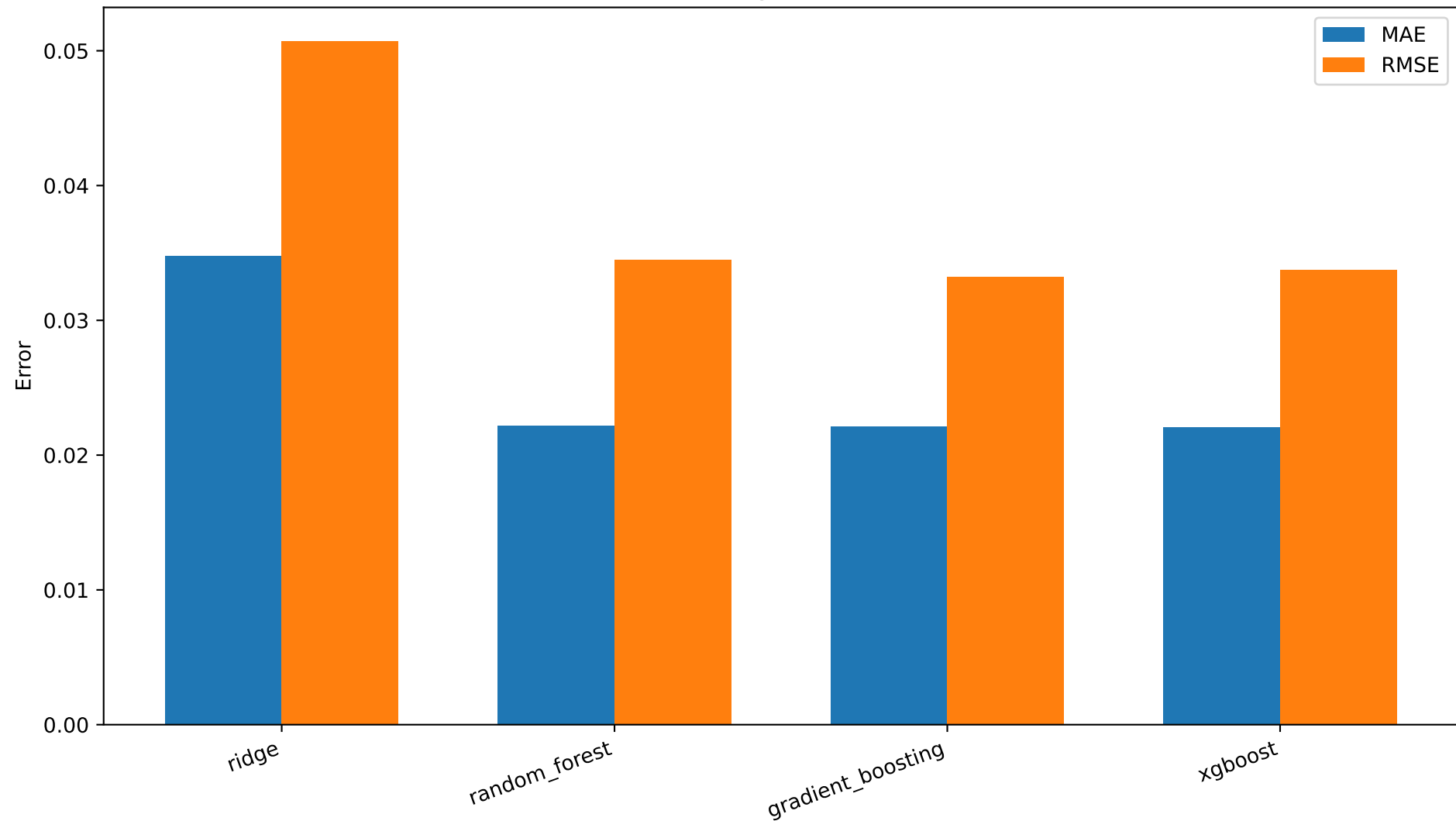
Meta-Learning Prediction Error
