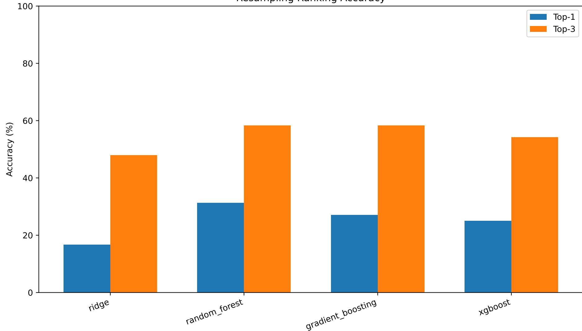
Resampling Ranking Accuracy
