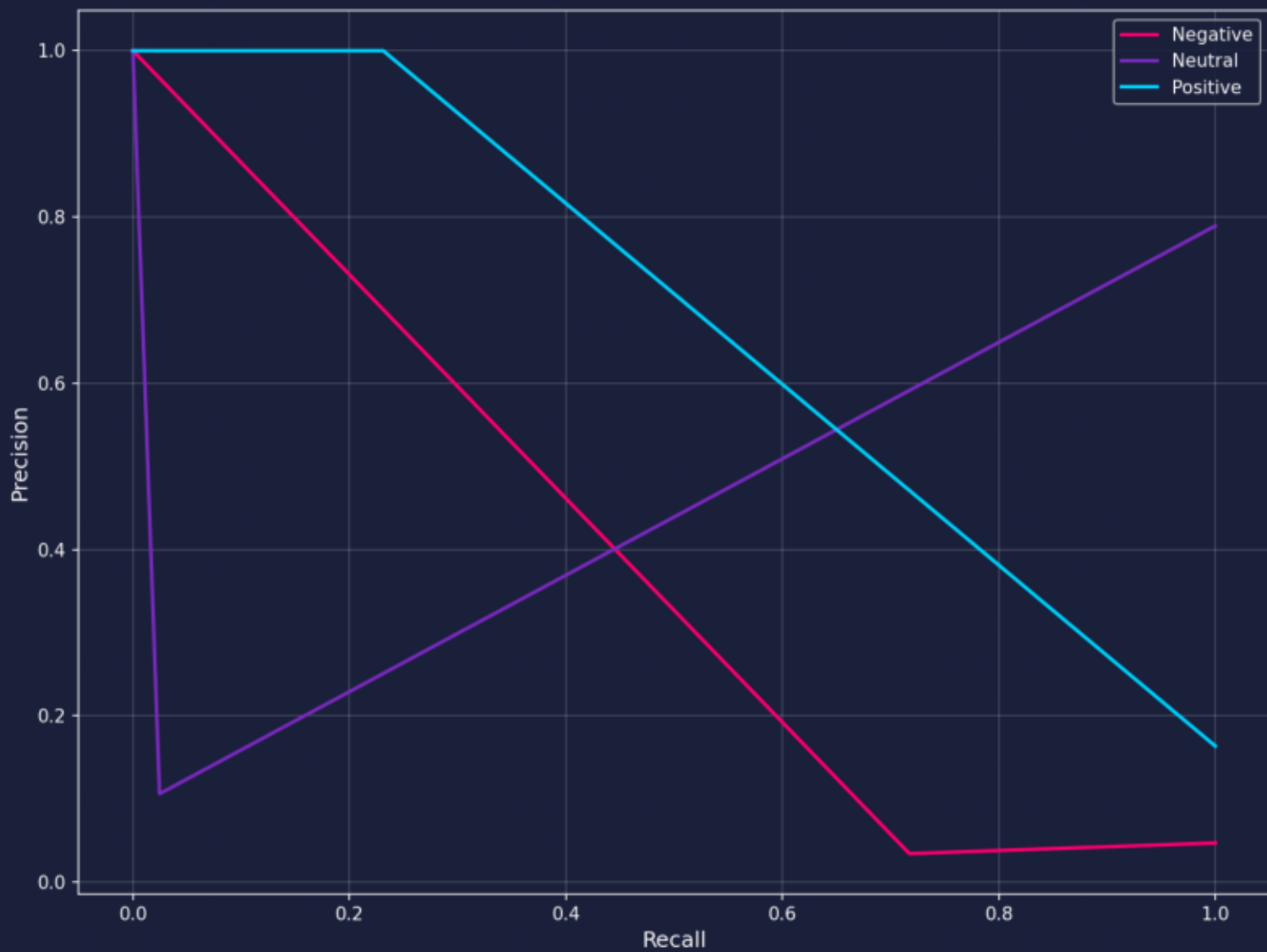
Precision-Recall Curve
