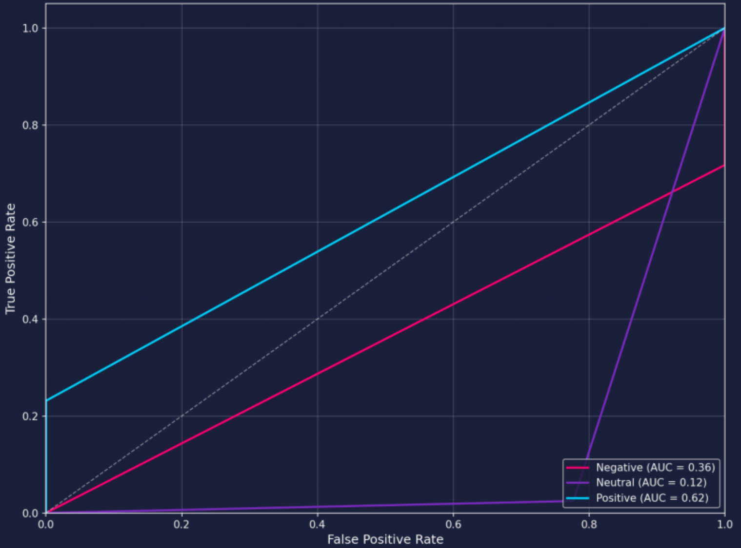
ROC Curve - Multiclass Sentiment
