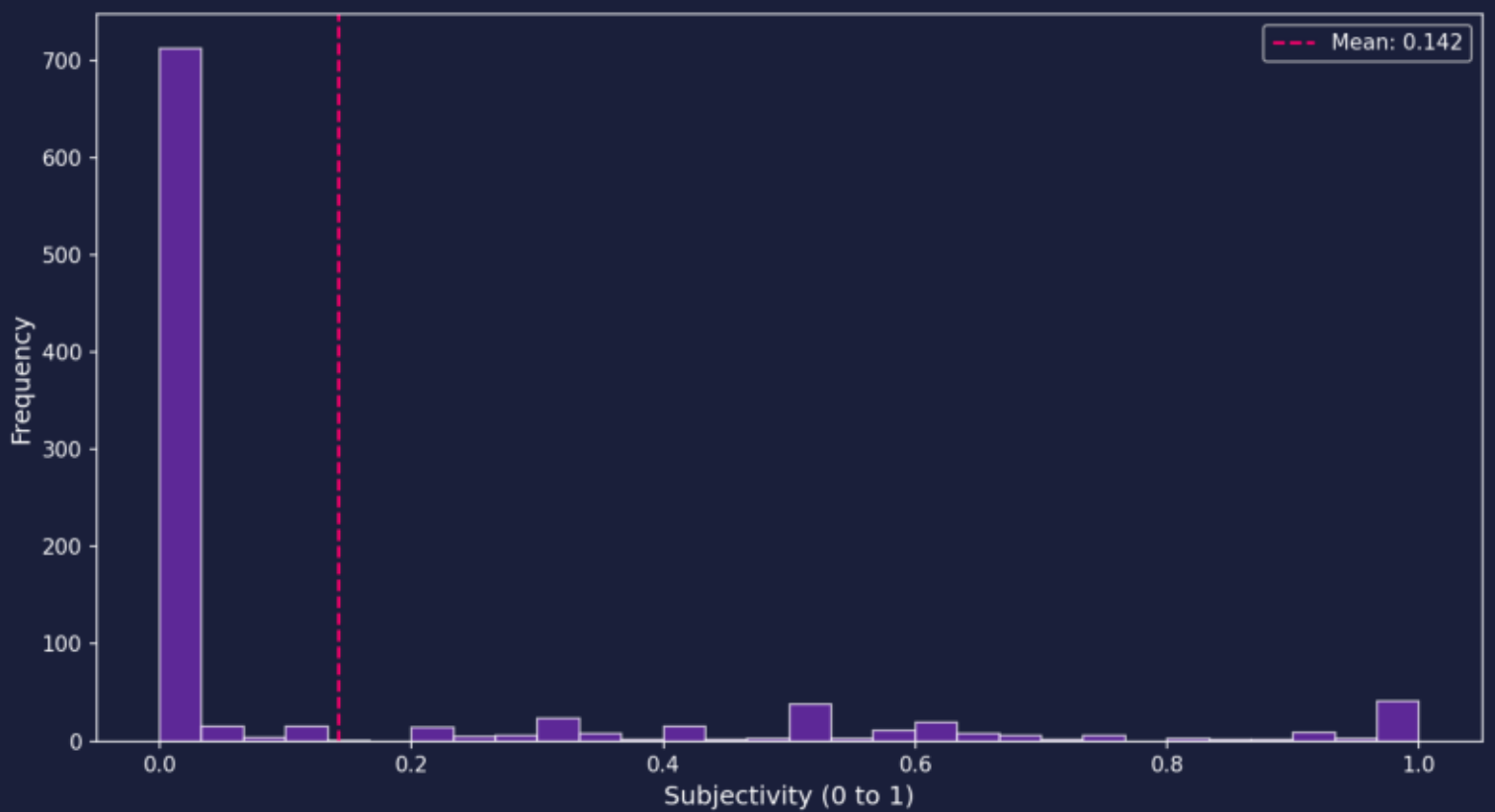
Subjectivity Distribution
