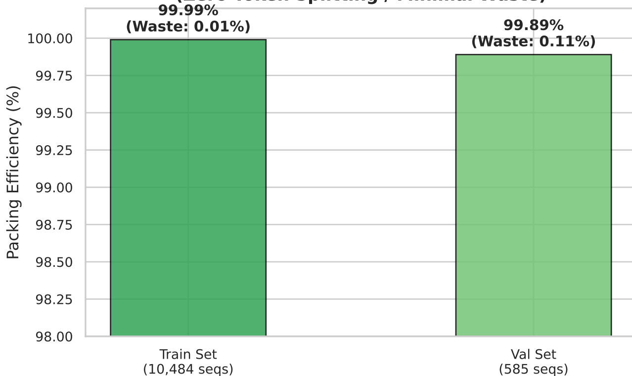
512-Token Sequence Packing Efficiency (Zero Token Splitting / Minimal Waste)
