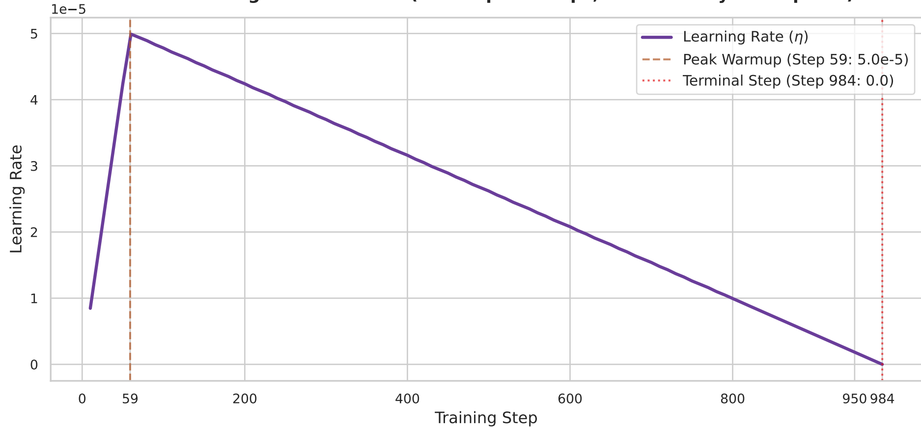
DAPT Learning Rate Schedule (Warmup: 59 steps, Linear Decay to Step 984)
