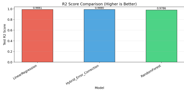
FIGURE 2. R^2 comparison across models. Linear Regression and the Hybrid Residual model explain nearly identical variance, while Random Forest explains less. The key insight is that global variance is dominated by the deterministic renewable-generation structure, which both the linear baseline and the residual model capture effectively. Residual learning should complement, not discard, the interpretable baseline.
