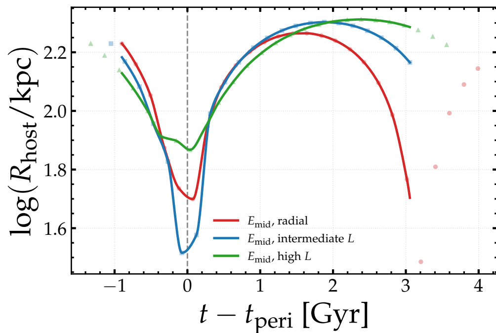
Orbital radius
