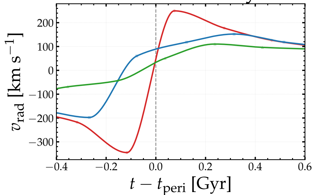
Radial velocity
