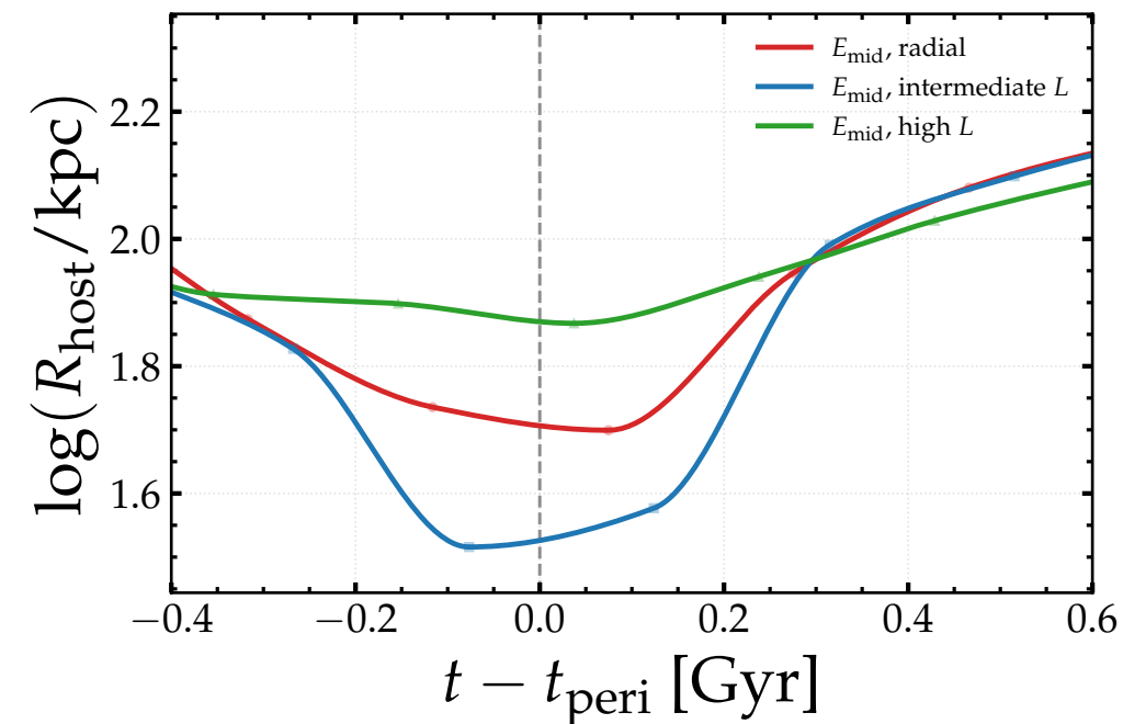
Orbital radius
