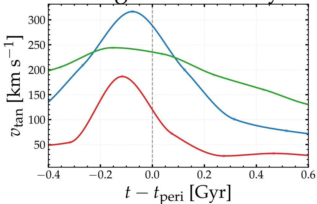
Tangential velocity
