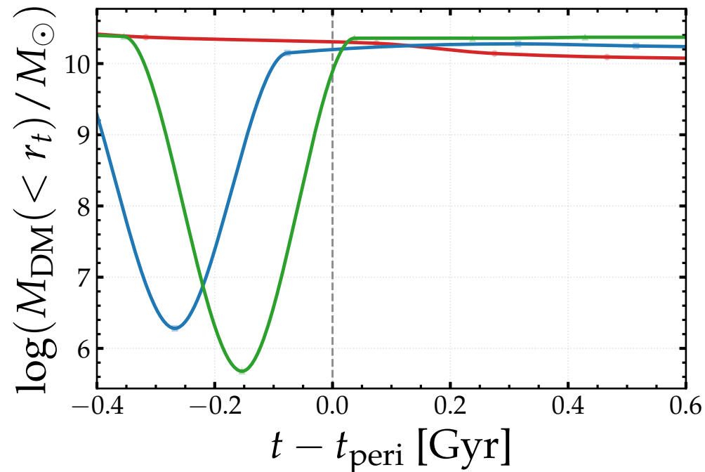
Dark matter mass inside tidal radius
