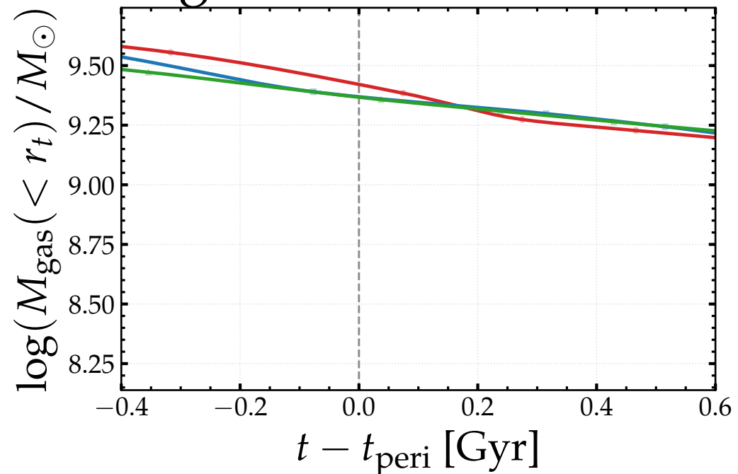
Satellite gas mass inside tidal radius
