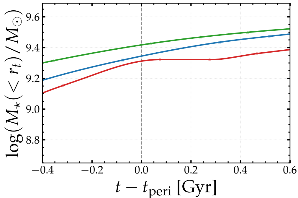
Stellar mass inside tidal radius
