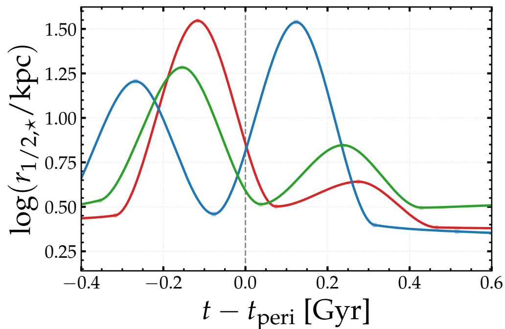
Stellar half-mass radius
