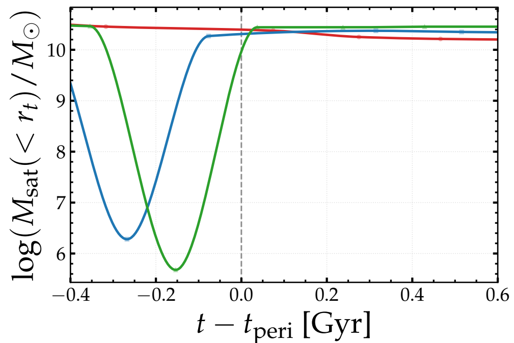
Total mass inside tidal radius
