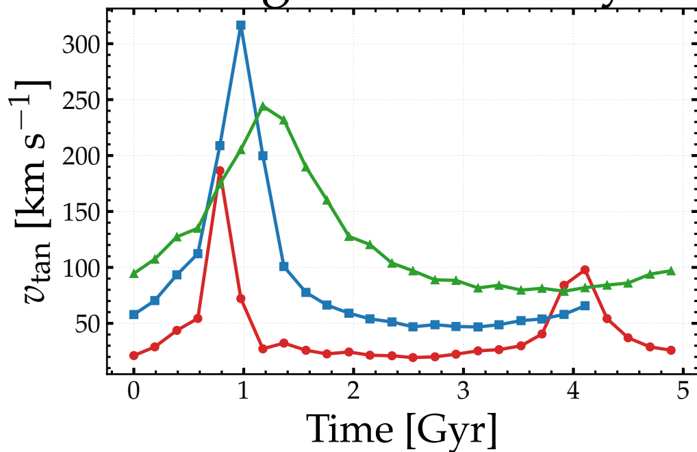
Tangential velocity
