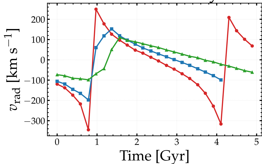
Radial velocity
