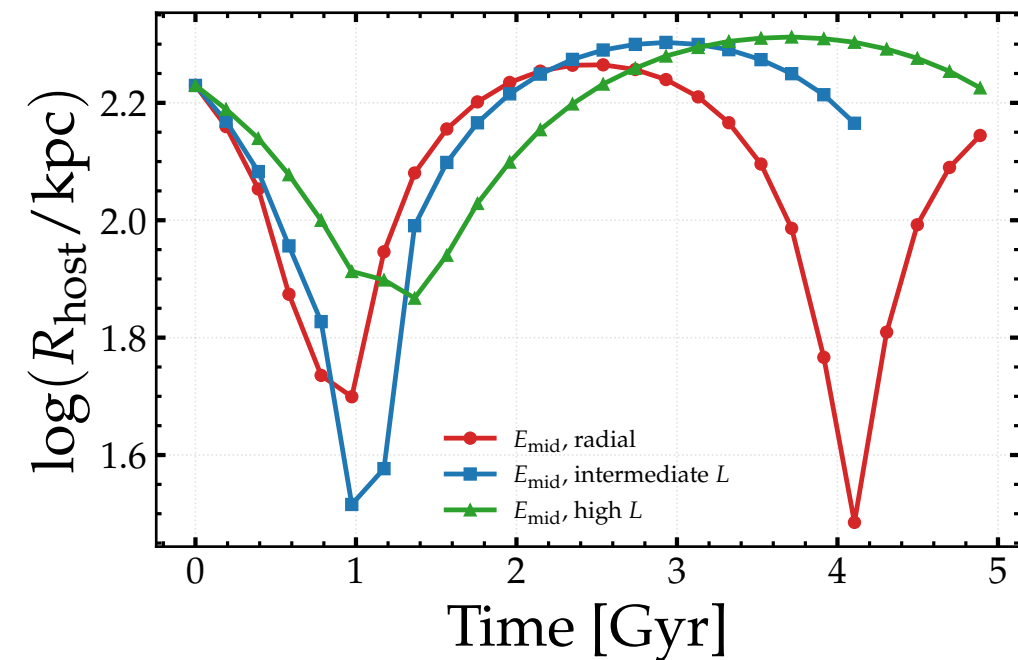
Orbital radius
