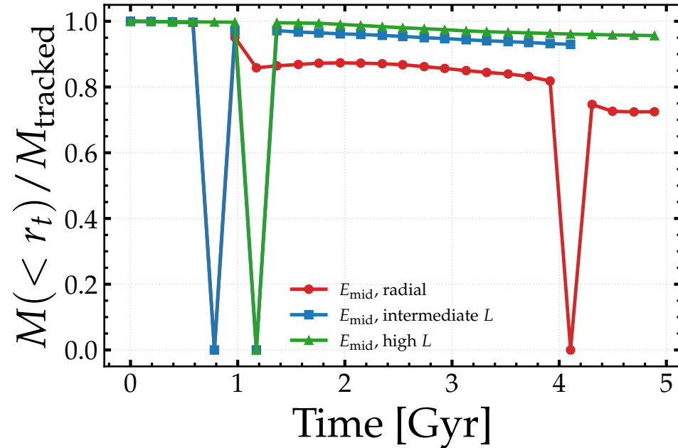
stars
