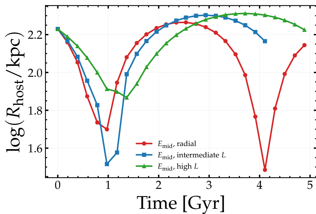
Orbital radius
