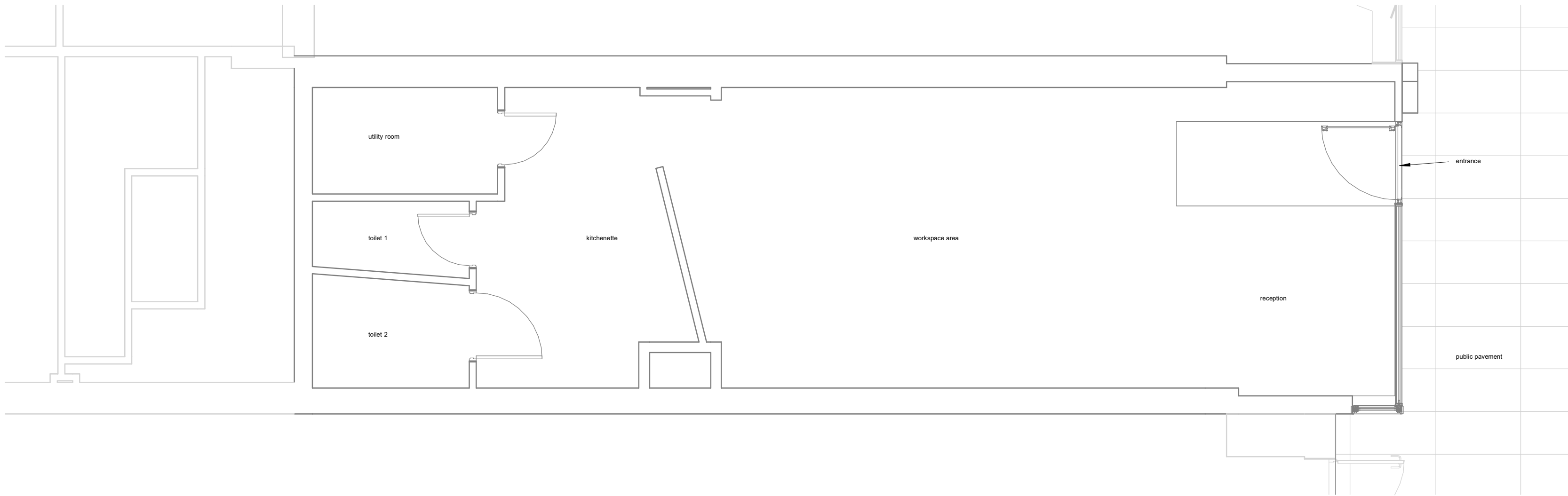
Existing Ground Floor
