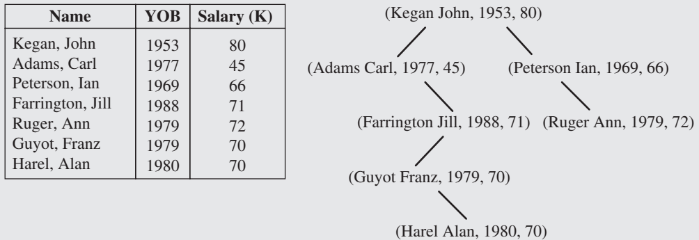
FIGURE 6.62 An example of a 3-d tree.
