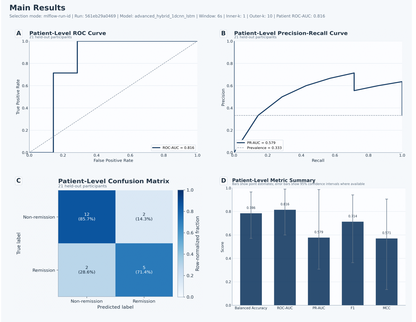
Figure 3: Best-run main-results composite for the hybrid model. The figure summarizes the patient-level ROC curve, PR curve, confusion matrix, and metric summary for the highest-performing sweep setting.
