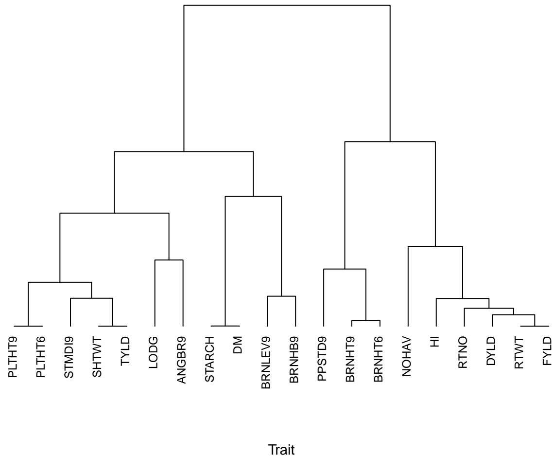
Dendrogram. Environment: Ikenne Ward method
