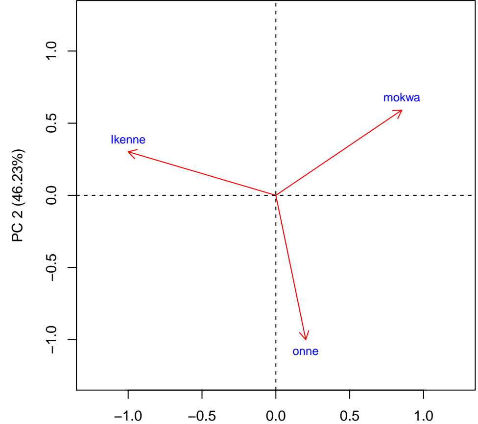
Biplot. Trait: FYLD
