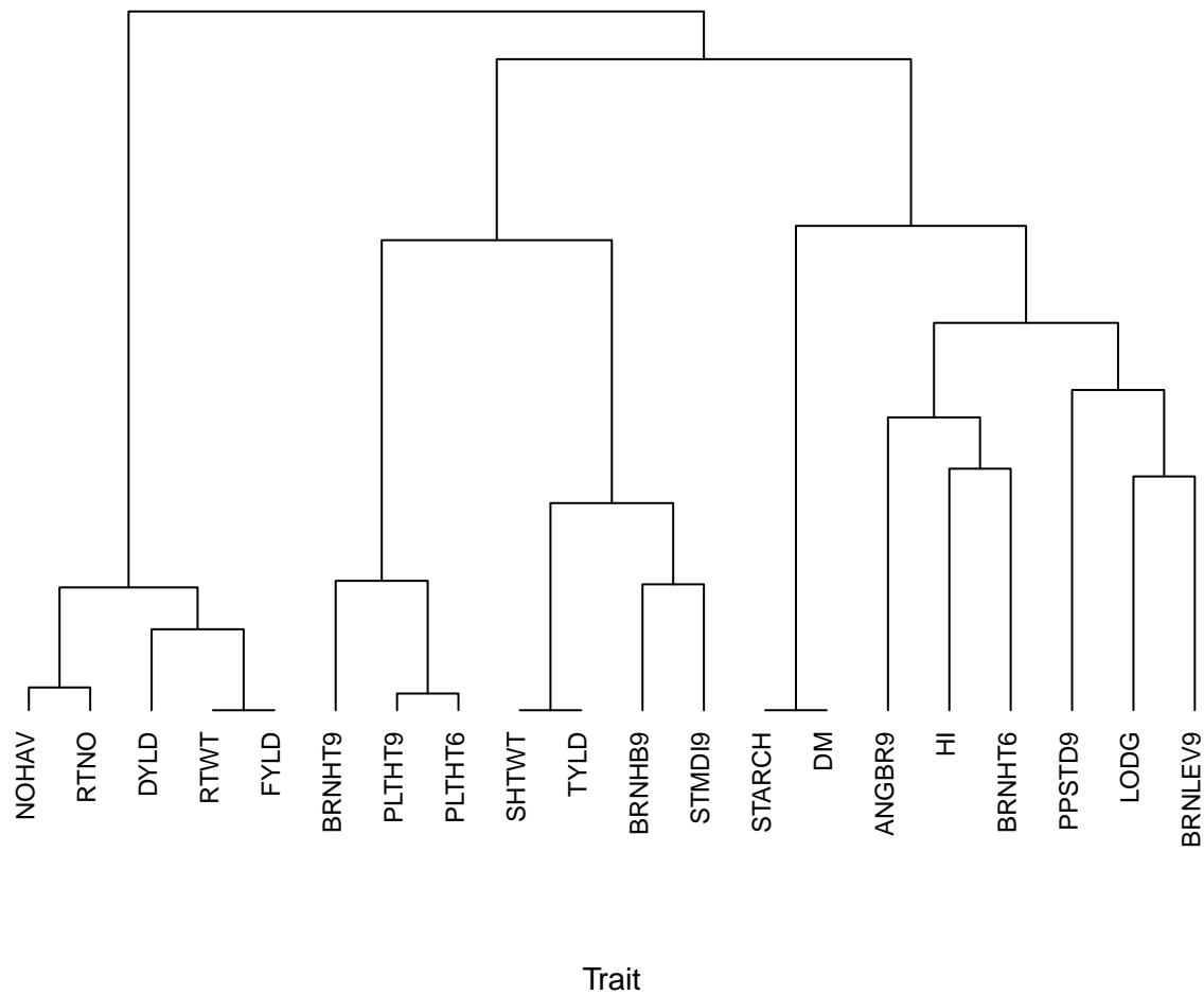
Dendrogram. Environment: onne Ward method
