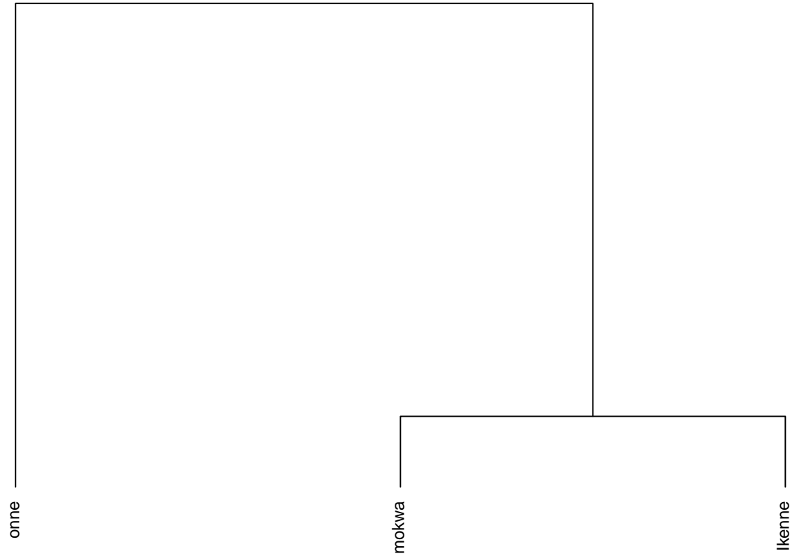
Dendrogram. Trait: BRNHT6 Ward method
