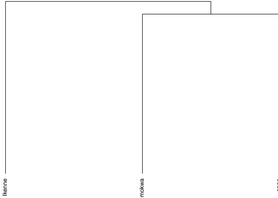
Dendrogram. Trait: FYLD Ward method
