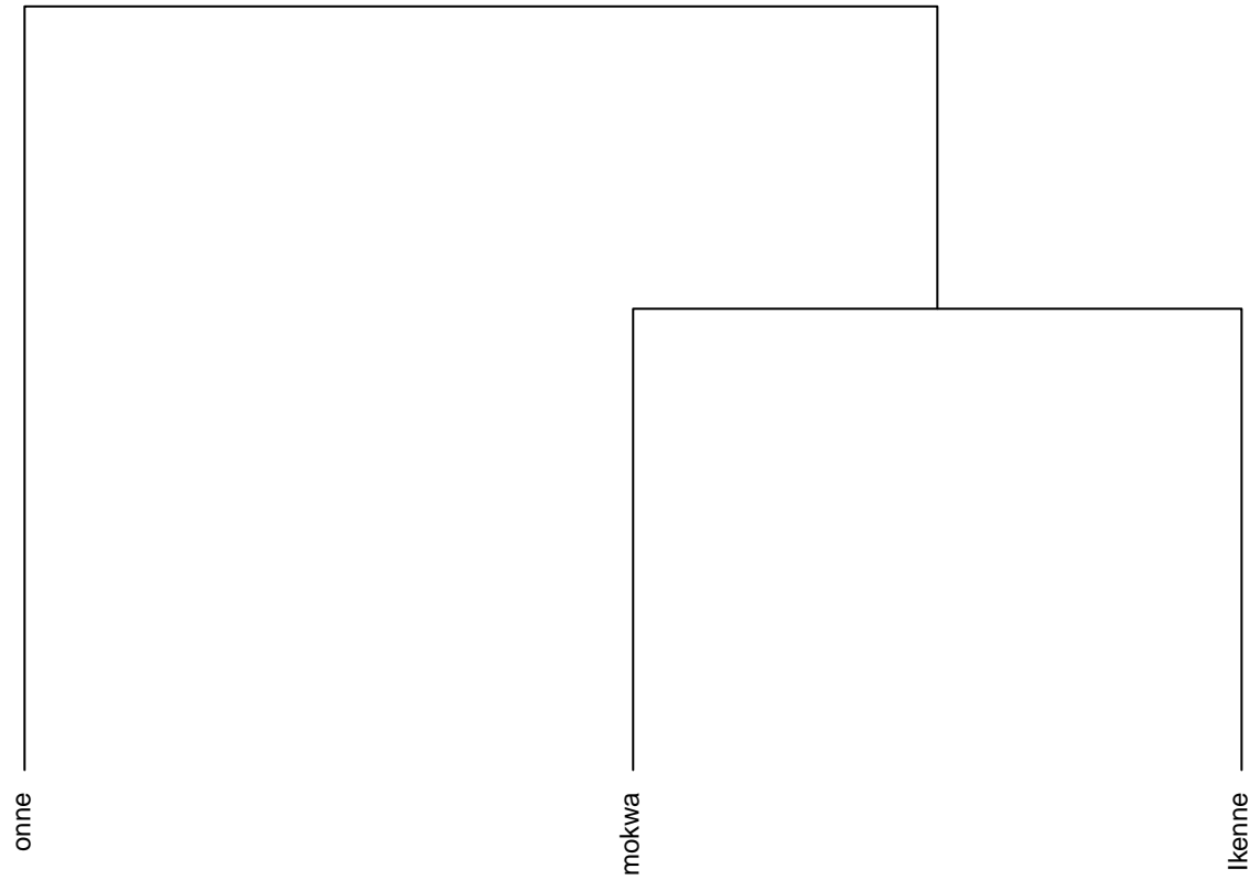
Dendrogram. Trait: STMDI9 Ward method
