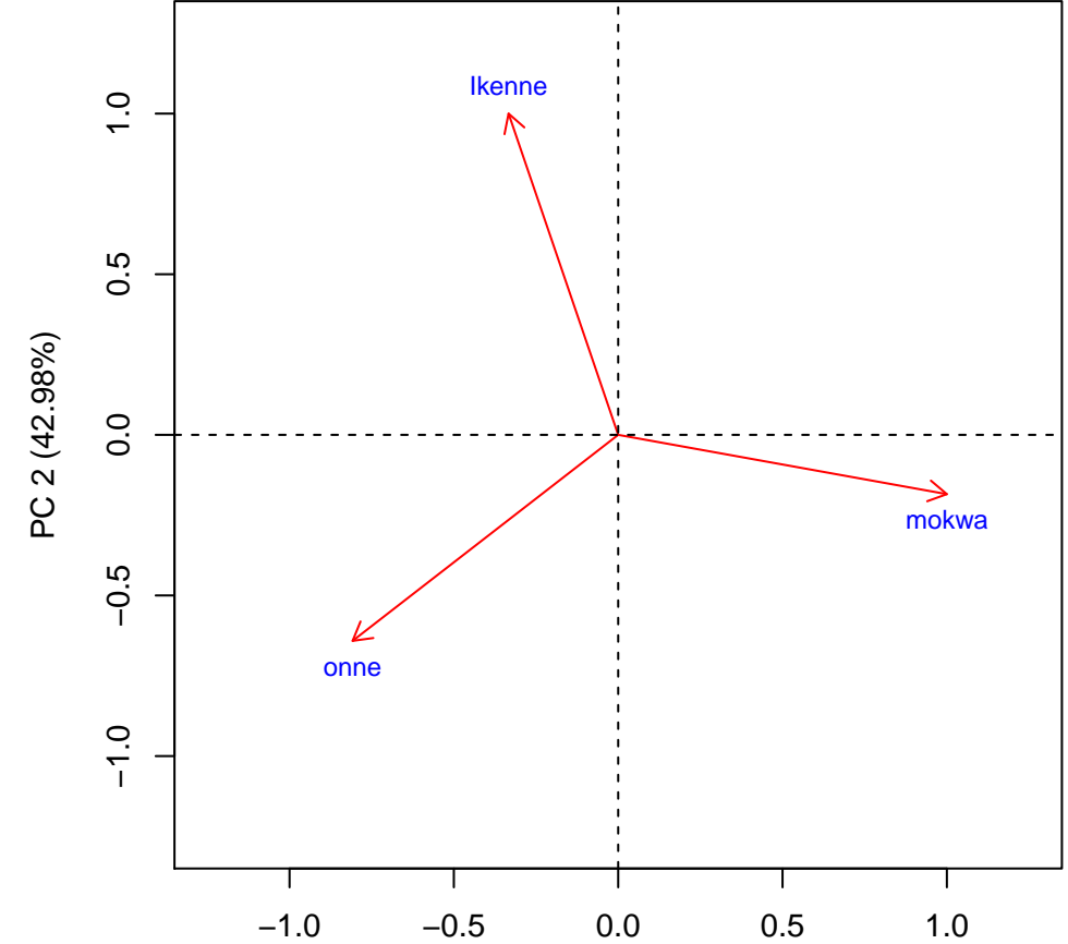
Biplot. Trait: DM
