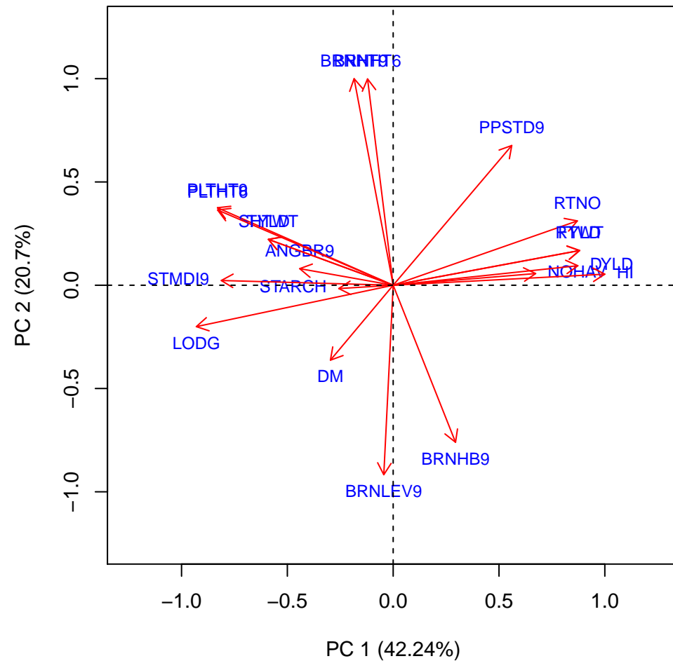
Biplot. Environment: Ikenne
