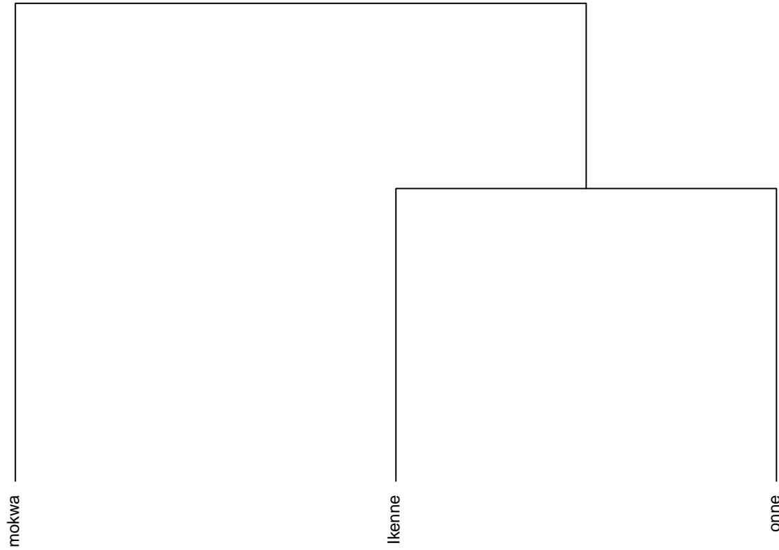
Dendrogram. Trait: SHTWT Ward method
