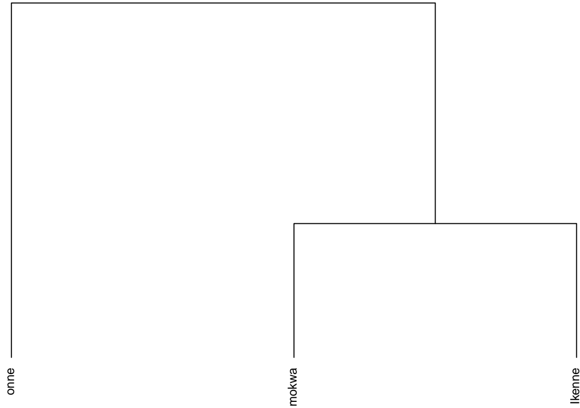
Dendrogram. Trait: PLTHT9 Ward method
