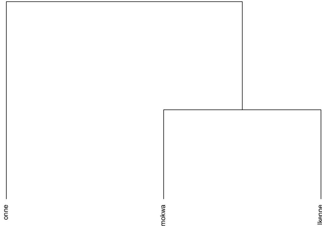
Dendrogram. Trait: LODG Ward method
