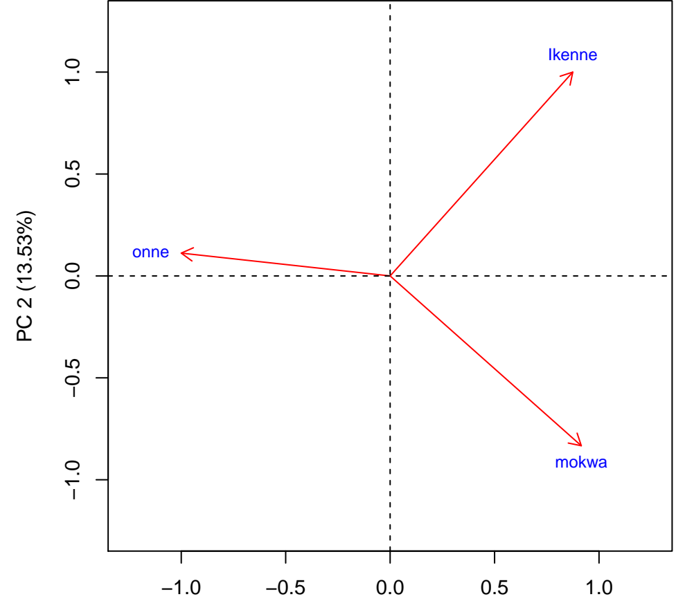
Biplot. Trait: PLTHT9
