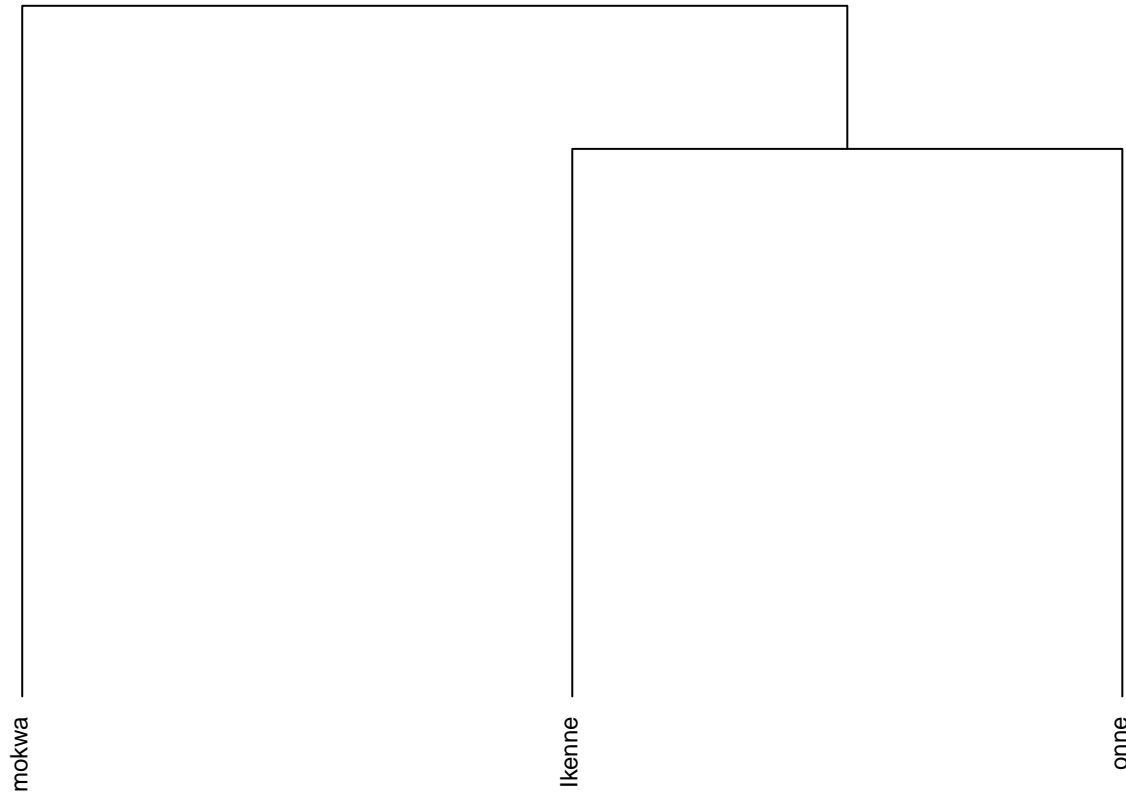
Dendrogram. Trait: STARCH Ward method
