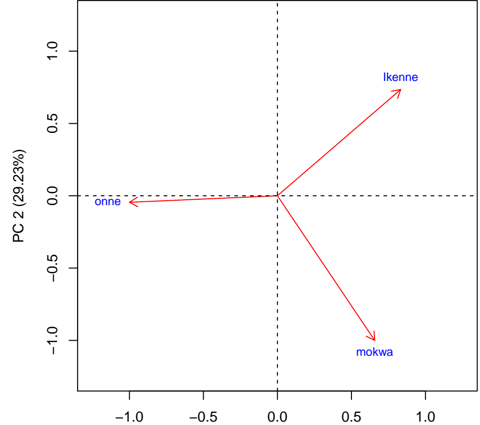
Biplot. Trait: STMDI9
