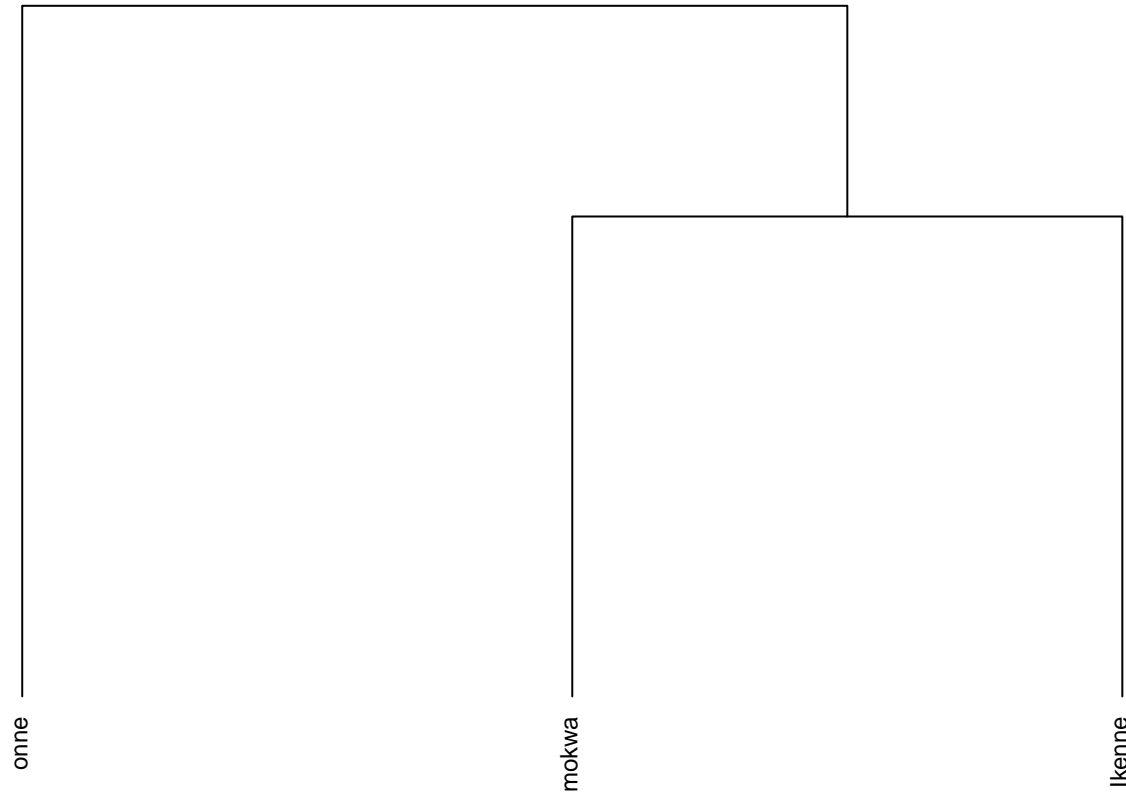
Dendrogram. Trait: ANGBR9 Ward method
