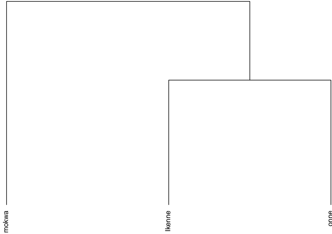
Dendrogram. Trait: TYLD Ward method
