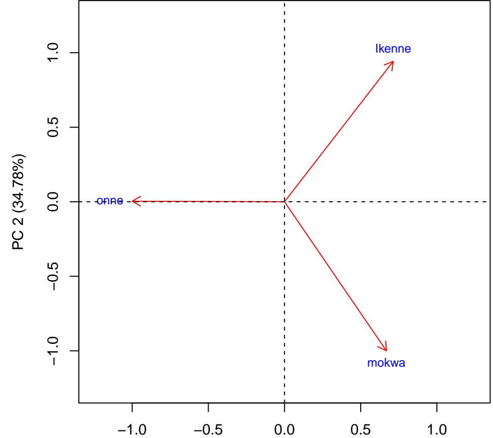
Biplot. Trait: ANGBR9
