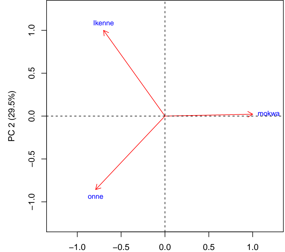
Biplot. Trait: SHTWT
