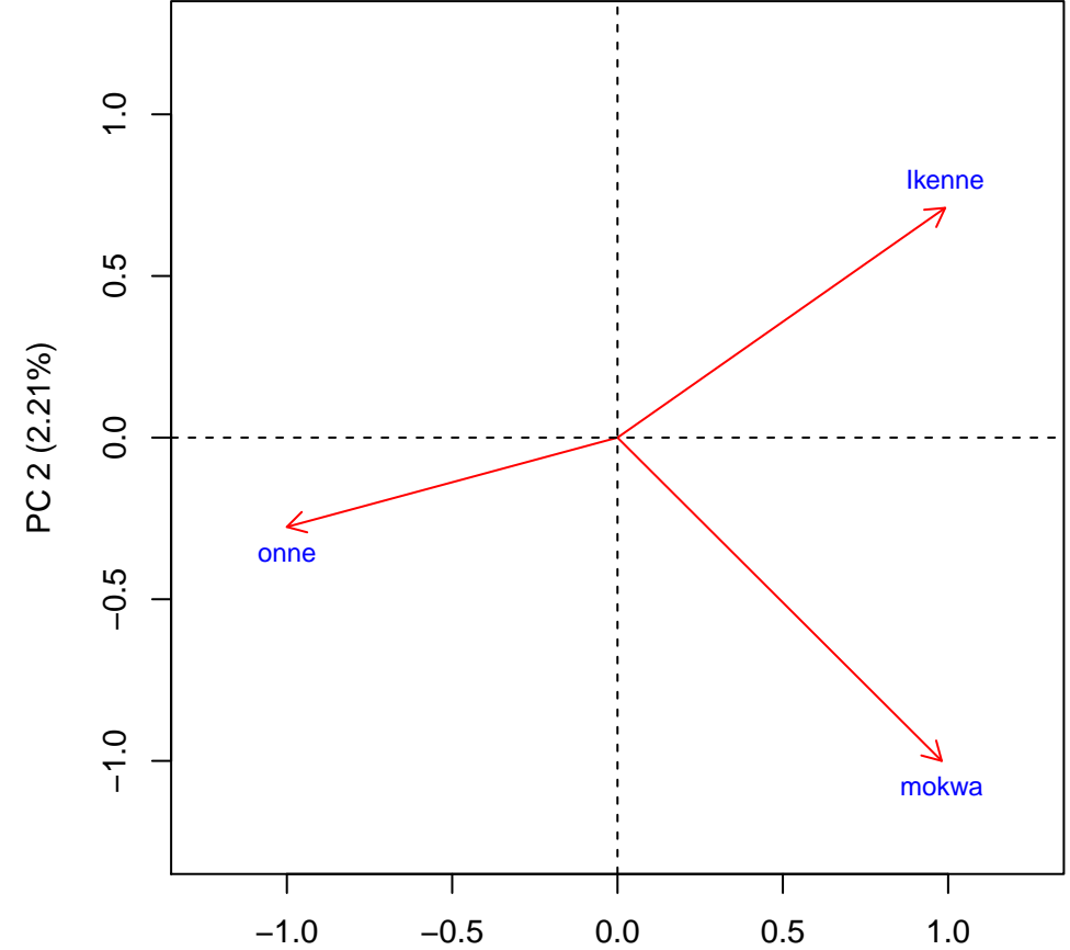
Biplot. Trait: BRNHT6
