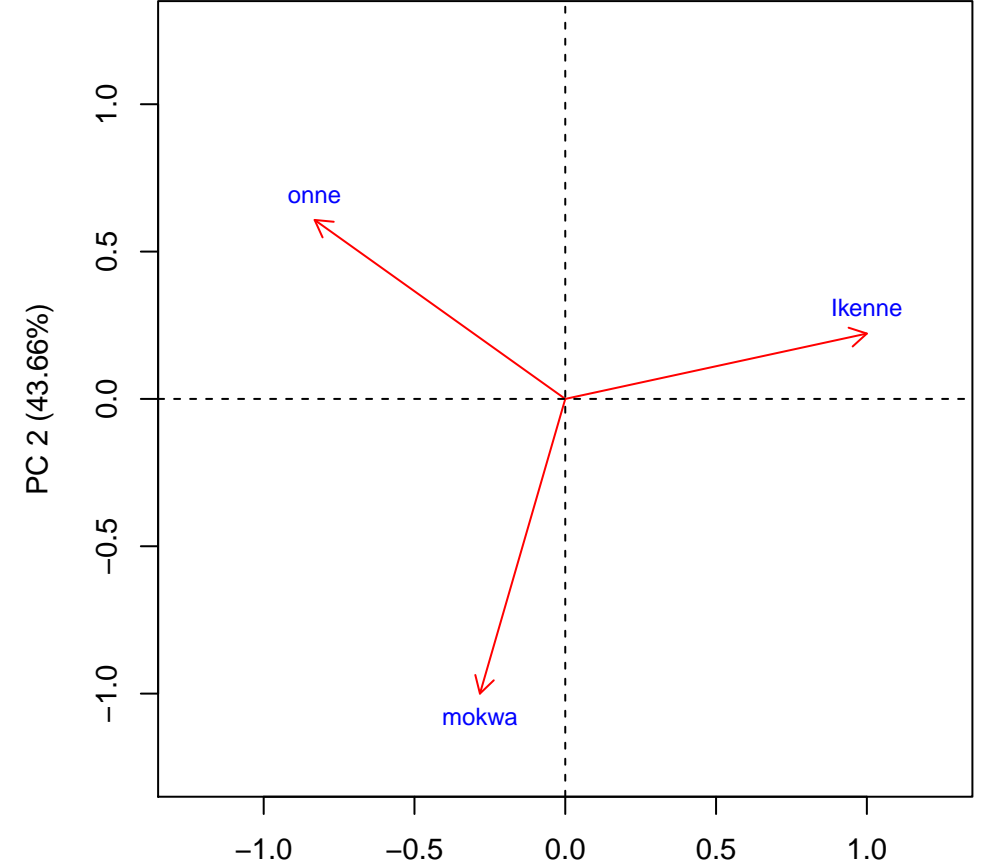
Biplot. Trait: RTNO
