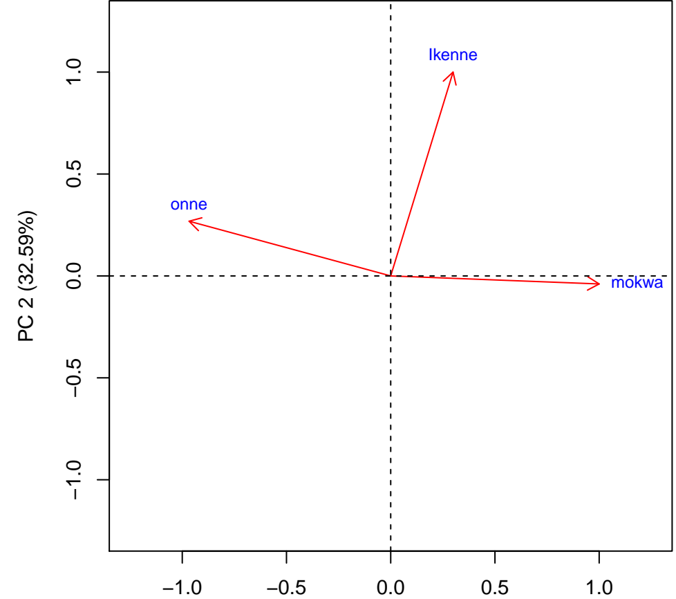
Biplot. Trait: LODG
