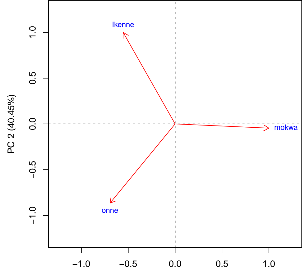
Biplot. Trait: STARCH
