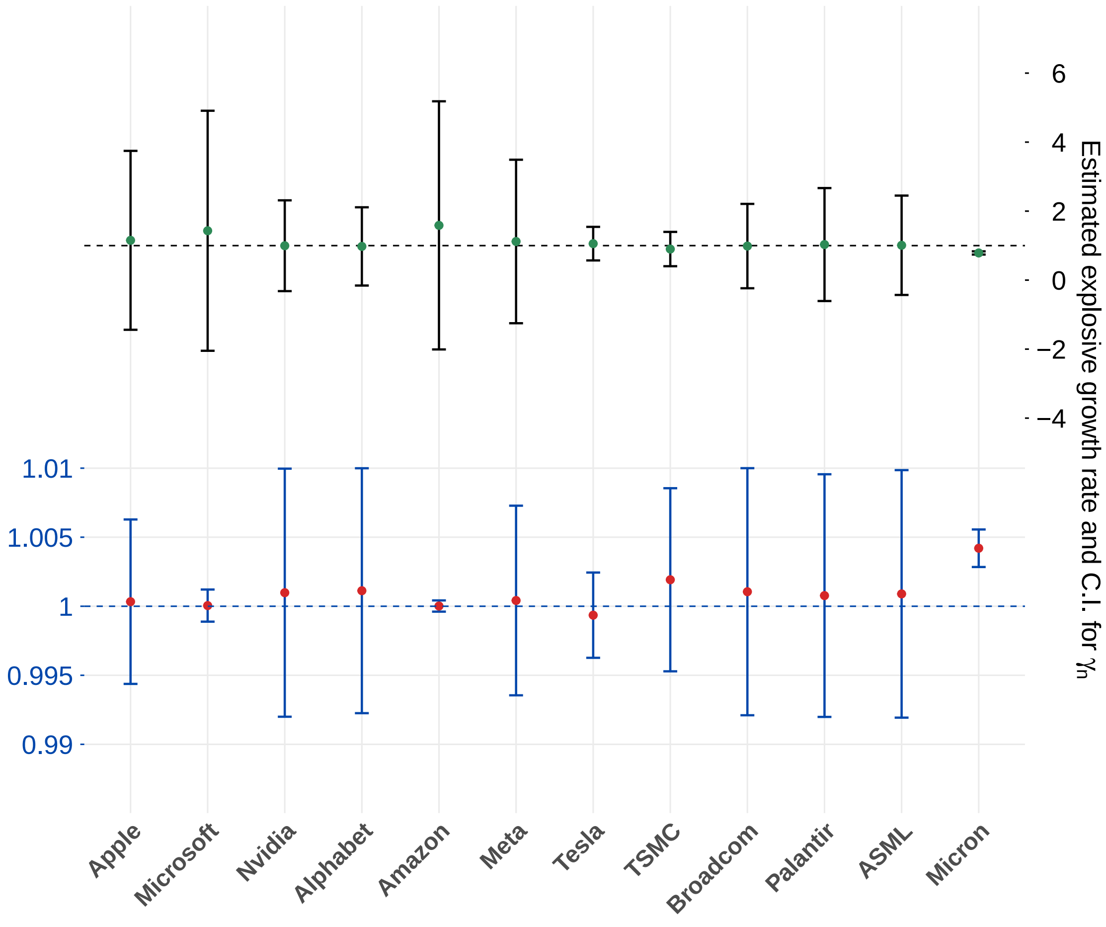
Estimated AR coefficient and C.I. for \delta_n
