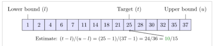
Visualization of interpolation search using linear interpolation. In this case, no searching is needed because the estimate of the target's location within the array is correct. Other implementations may specify another function for estimating the target's location.
