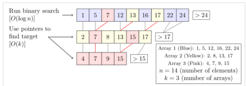
In fractional cascading, each array has pointers to every second element of another array, so only one binary search has to be performed to search all the arrays.
