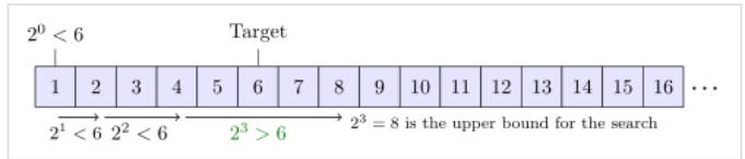
Visualization of exponential searching finding the upper bound for the subsequent binary search
