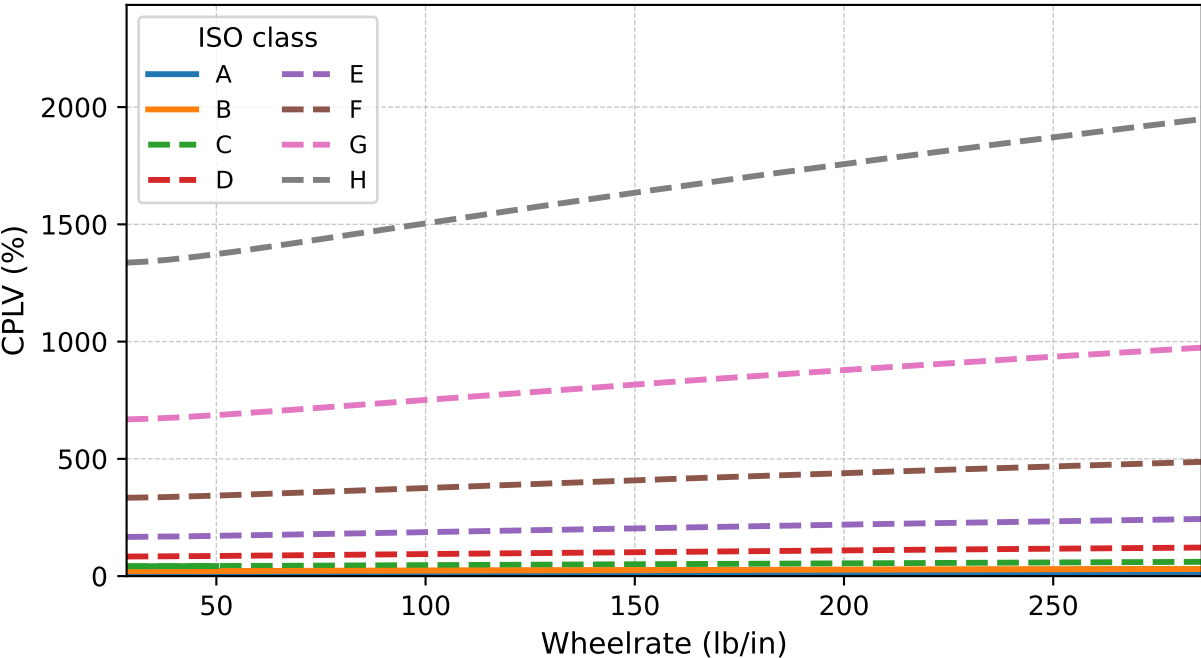
Front corner | contact-load variation
