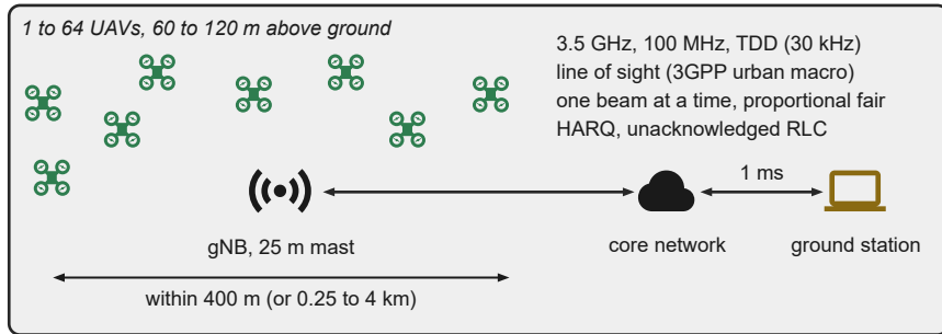
b 5G NR cell (5G-LENA): what the test bed cannot show
