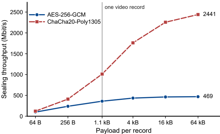
(a) Raspberry Pi 4B: AES in software
