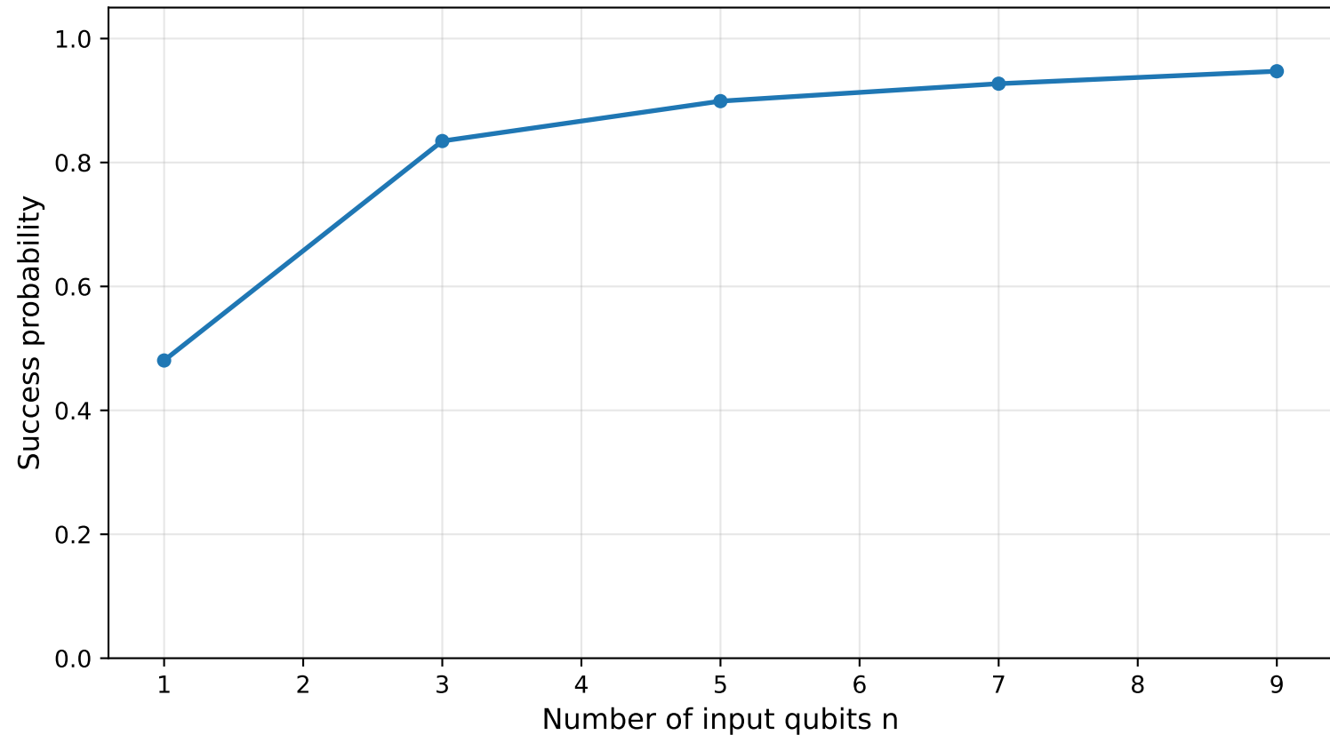
Scalability for balanced under R_X(\theta) at E_4 noise axis=X, \theta=90^\circ , shots=1024
