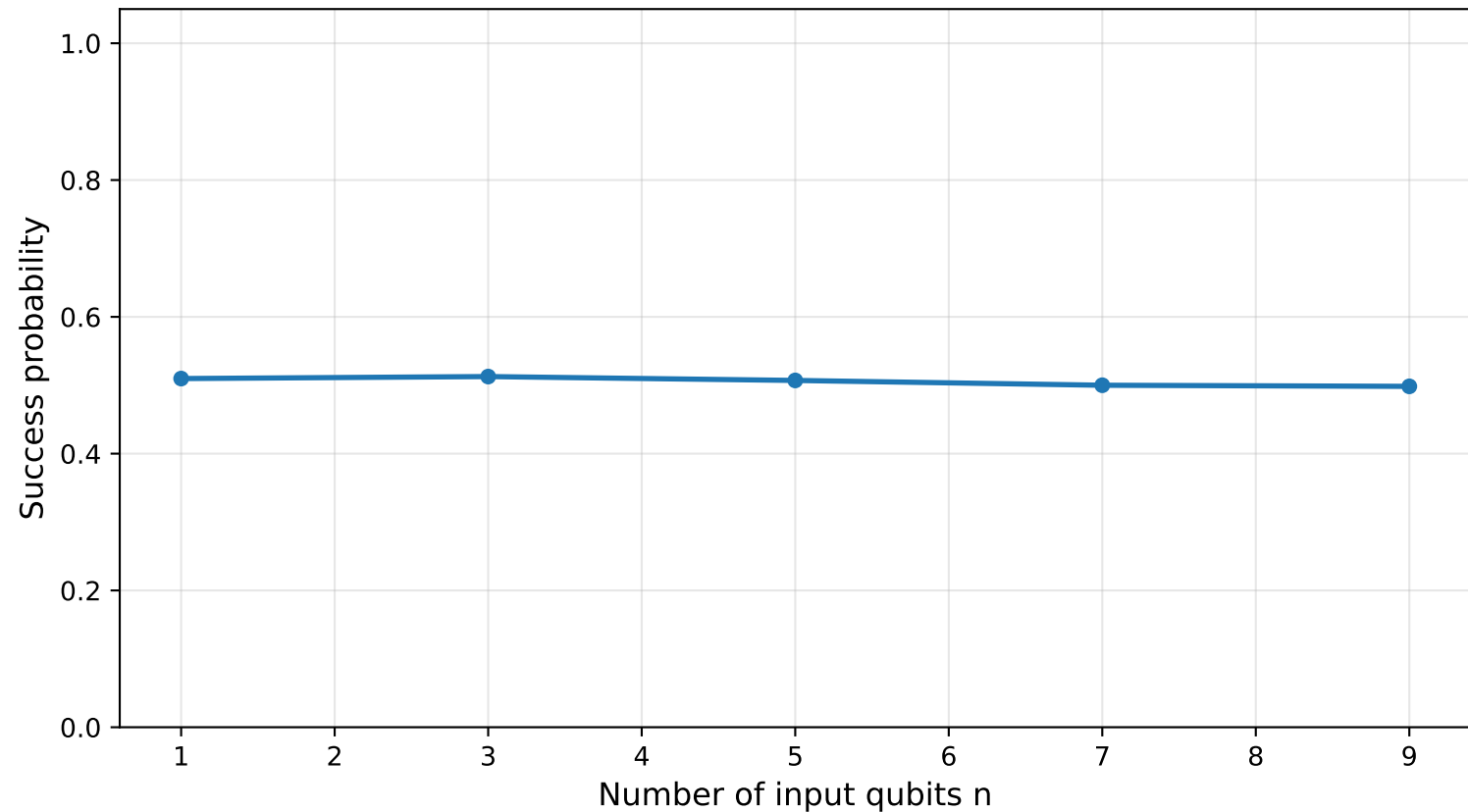
Scalability for constant_0 under R_X(\theta) at E_4 noise axis=X, \theta=90^\circ , shots=1024
