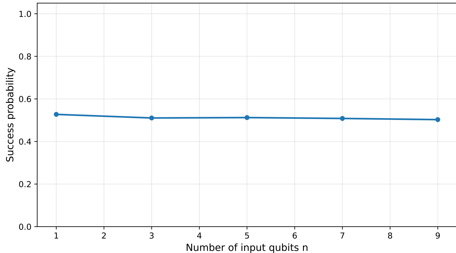
Scalability for constant_0 under R_Y(\theta) at E_4 noise axis=Y, \theta=90^\circ , shots=1024
