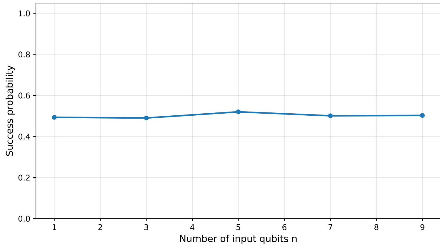
Scalability for constant_1 under R_Z(\theta) at E_3 noise axis=Z, \theta=90^\circ , shots=1024
