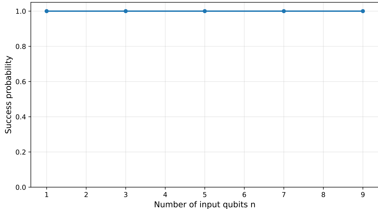
Scalability for constant_1 under R_Z(\theta) at E_4 noise axis=Z, \theta=90^\circ , shots=1024
