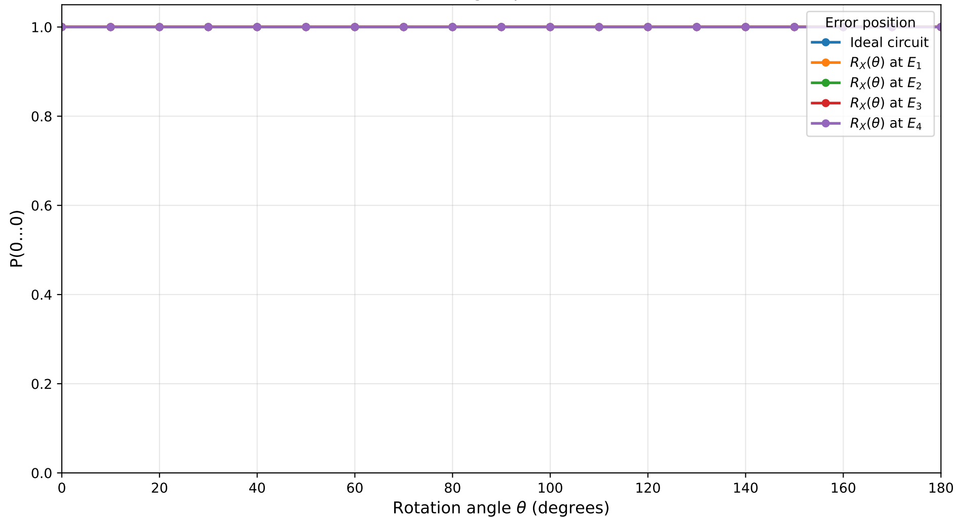
Probability under X-Axis Rotation Errors Balanced, n=9, target qubit=4, shots=1024
