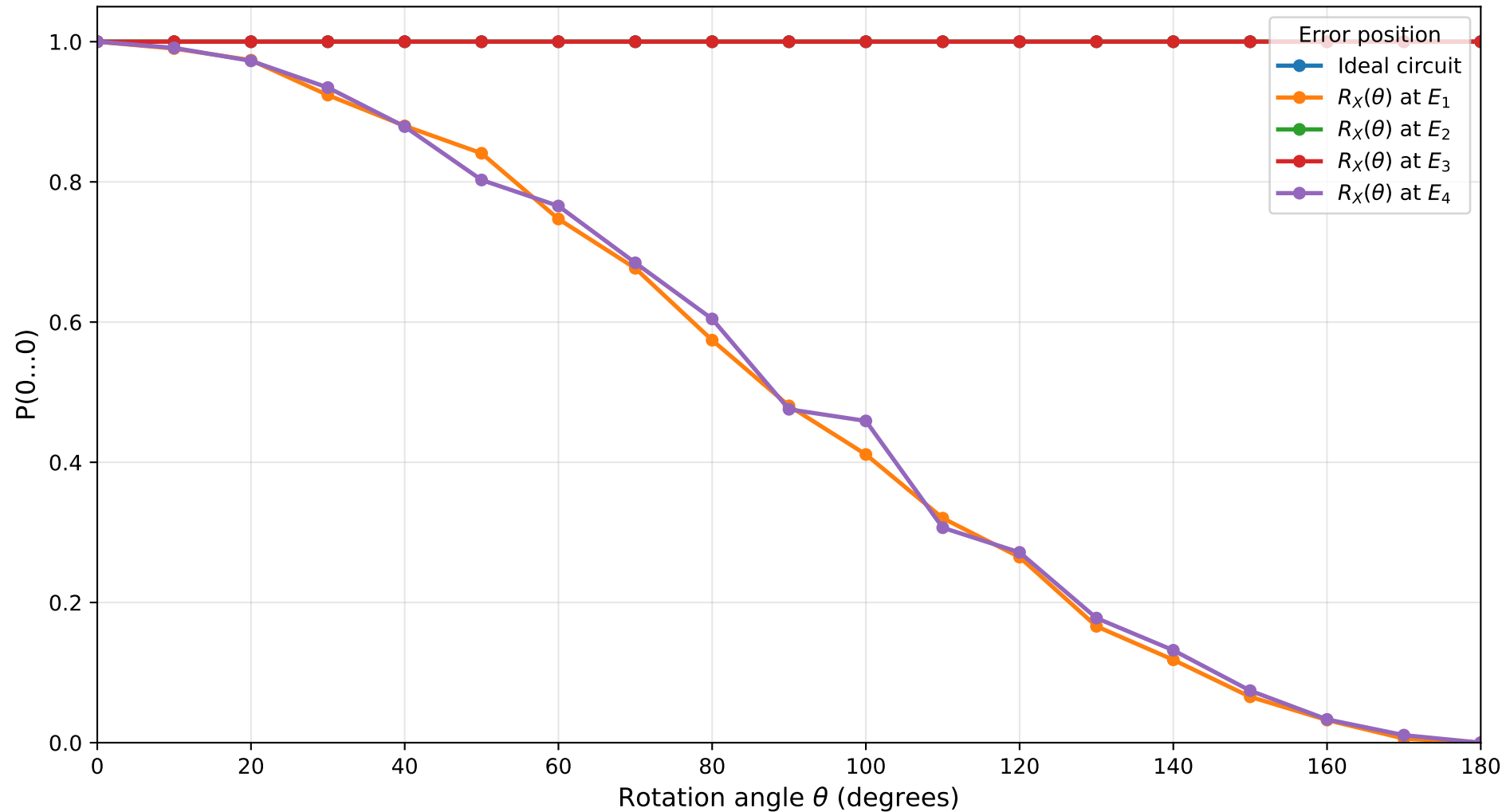
Probability under X-Axis Rotation Errors Constant 1, n=9 , target qubit=4, shots=1024
