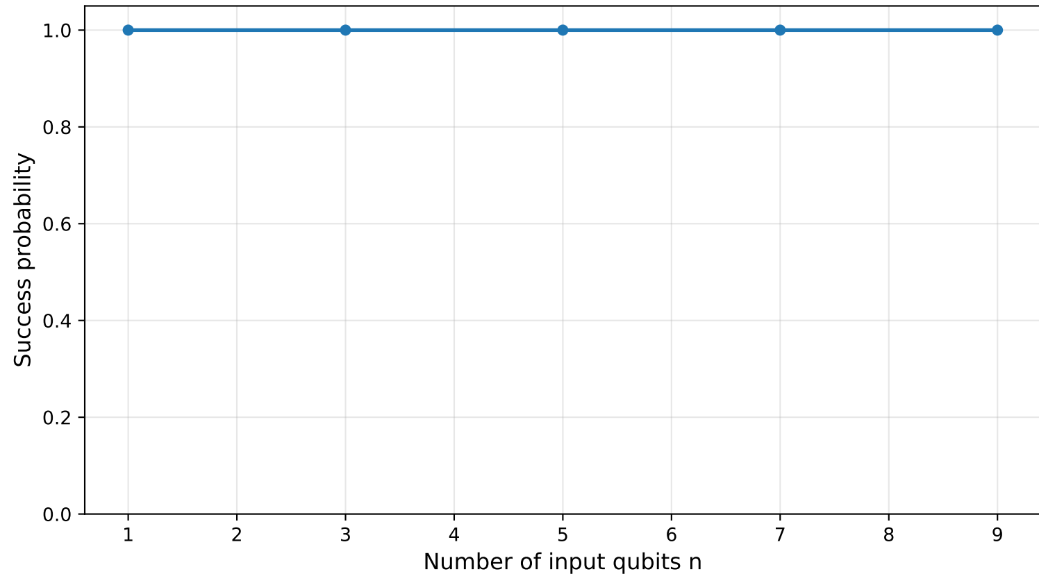
Scalability for balanced under R_X(\theta) at E_3 noise axis=X, \theta=90^\circ , shots=1024
