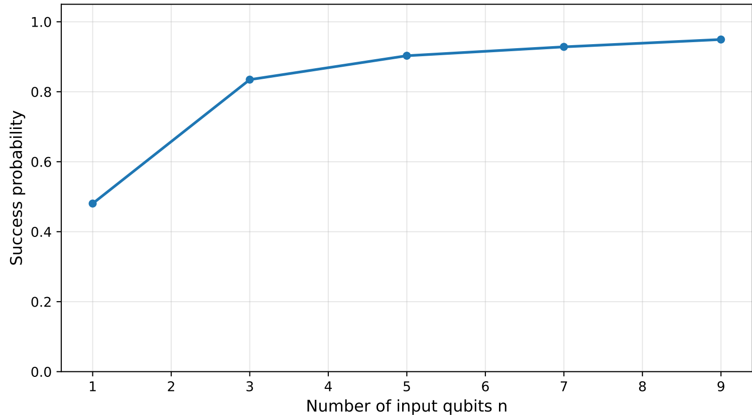
Scalability for balanced under R_Y(\theta) at E_4 noise axis=Y, \theta=90^\circ , shots=1024
