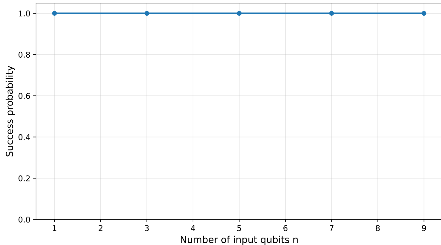
Scalability for constant_0 under R_Z(\theta) at E_4 noise axis=Z, \theta=90^\circ , shots=1024
