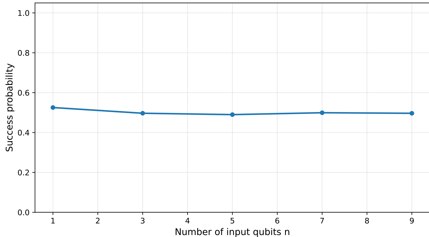
Scalability for constant_1 under R_Y(\theta) at E_3 noise axis=Y, \theta=90^\circ , shots=1024
