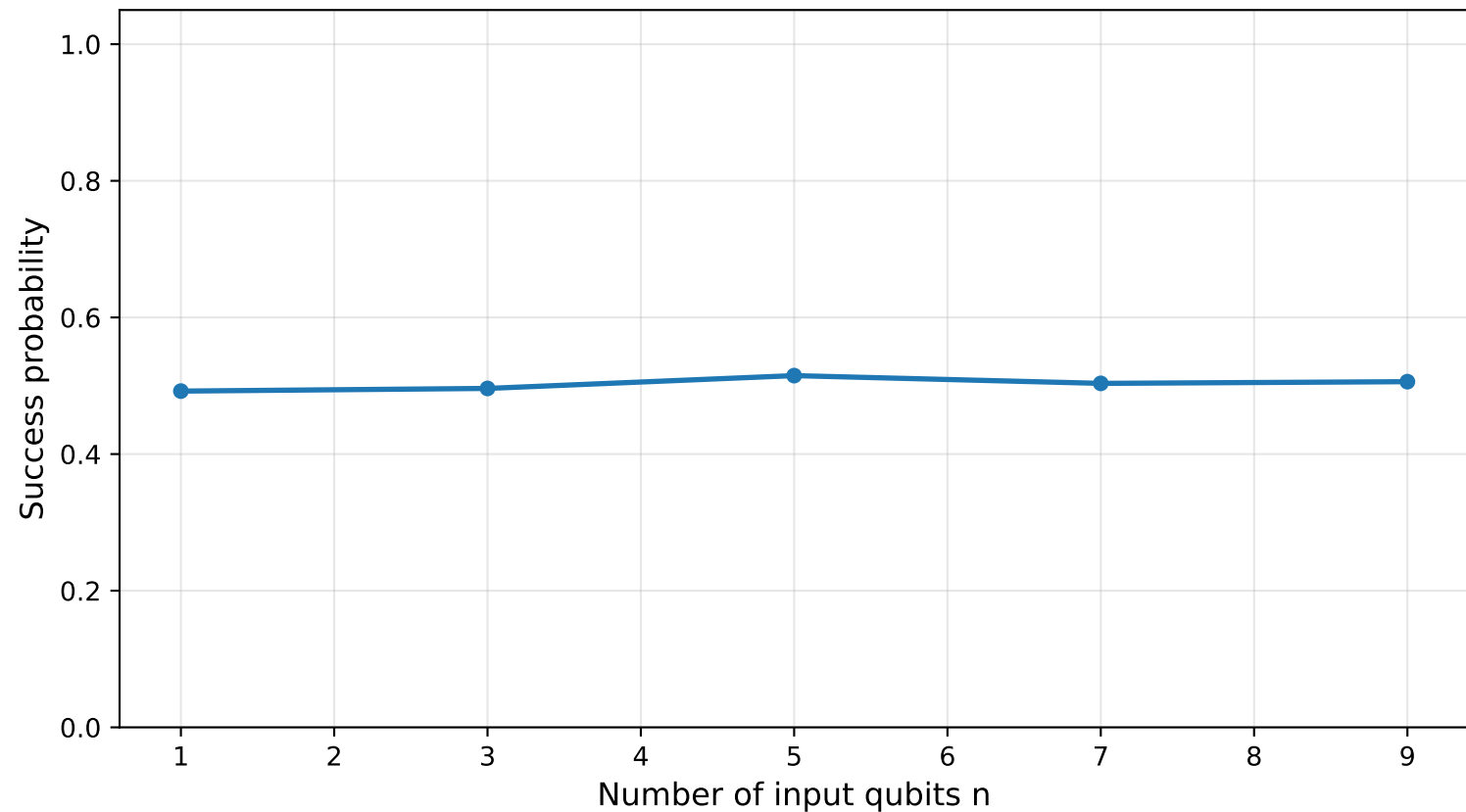
Scalability for constant_1 under R_X(\theta) at E_4 noise axis=X, \theta=90^\circ , shots=1024
