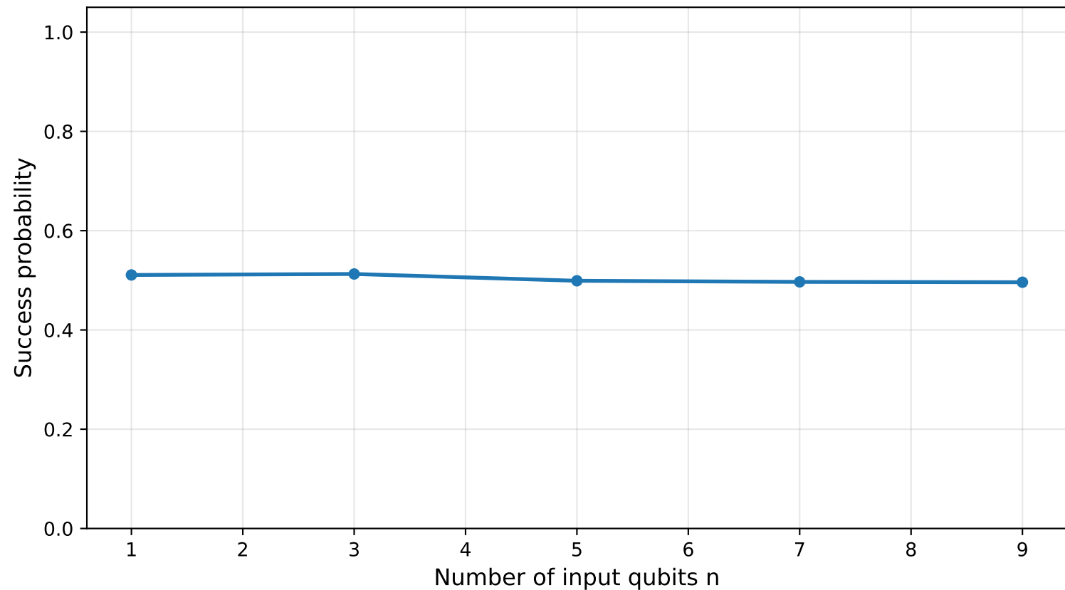
Scalability for constant_1 under R_Y(\theta) at E_4 noise axis=Y, \theta=90^\circ , shots=1024
