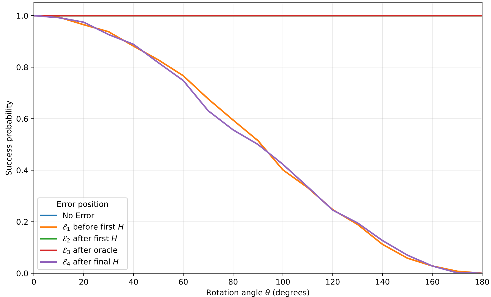
DJA success under rotation errors function=constant_1, n=9, axis=X, shots=1024
